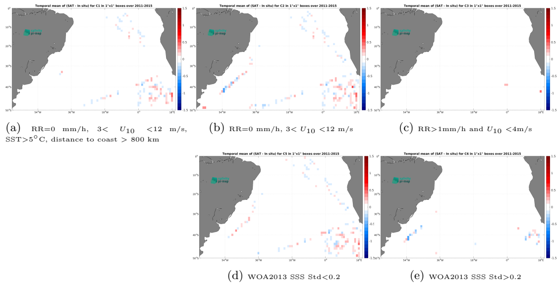
Figure 12: Temporal mean gridded over spatial boxes of size 1^\circ \times 1^\circ of \Delta\text{SSS} (Aquarius SSS L4 OI v5 - Weekly (IPRC) - TSG (Polarstern)) for 5 different subdatasets corresponding to:RR=0 mm/h, 3 < U_{10} < 12 m/s, SST >5^\circ\text{C} , distance to coast > 800 km (a), RR=0 mm/h, 3 < U_{10} < 12 m/s (b), RR >1 mm/h and U_{10} < 4 m/s (c), WOA2013 SSS Std <0.2 (d), WOA2013 SSS Std >0.2 (e).
