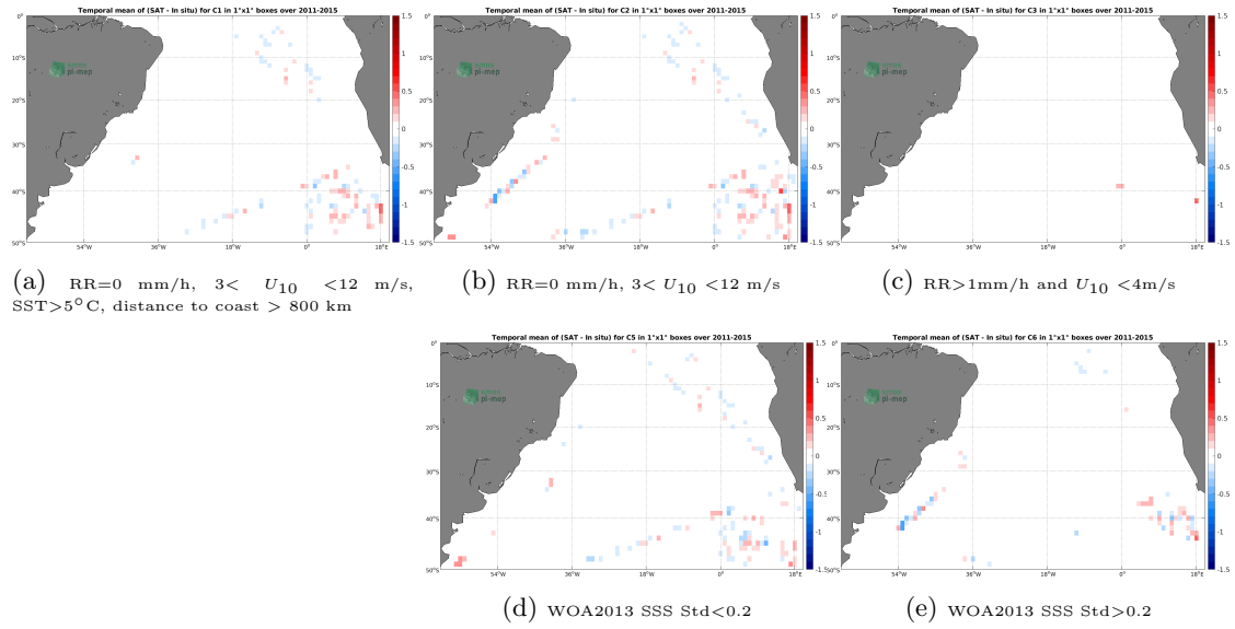
Figure 12: Temporal mean gridded over spatial boxes of size 1^\circ \times 1^\circ of \Delta SSS (Aquarius SSS L4 OI v5 - Weekly (IPRC) - TSG (Polarstern)) for 5 different subdatasets corresponding to: RR=0 mm/h, 3 < U_{10} < 12 m/s, SST > 5^\circ C , distance to coast > 800 km (a), RR=0 mm/h, 3 < U_{10} < 12 m/s (b), RR > 1 mm/h and U_{10} < 4 m/s (c), WOA2013 SSS Std < 0.2 (d), WOA2013 SSS Std > 0.2 (e).
