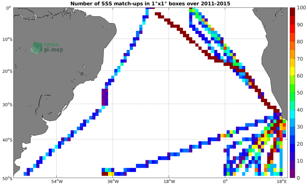
Figure 4: Number of SSS match-ups between TSG (Polarstern) SSS and the Aquarius SSS L4 OI v5 - Weekly (IPRC) SSS product for the South Atlantic Ocean Pi-MEP region over 1^\circ \times 1^\circ boxes and for the full satellite product period.
