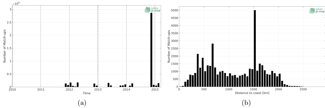
Figure 1: Number of match-ups between TSG (Polarstern) and Aquarius SSS L4 OI v5 - Weekly (IPRC) SSS as a function of time (a) and as function of the distance to coast (b) over the South Atlantic Ocean Pi-MEP region and for the full satellite product period.
