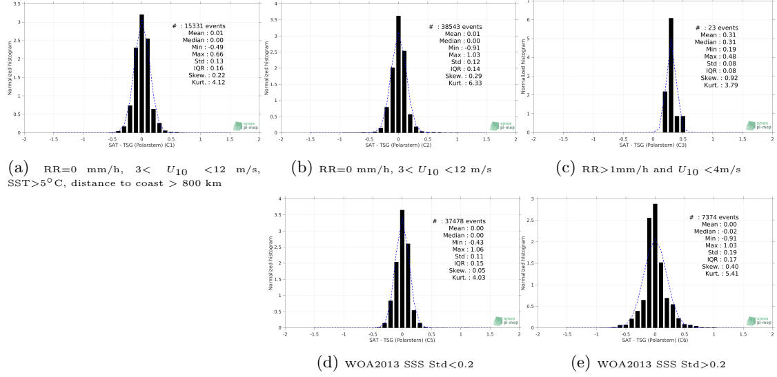
Figure 13: Normalized histogram of \Delta\text{SSS} (Aquarius SSS L4 OI v5 - Weekly (IPRC) - TSG (Polarstern)) for 5 different subdatasets corresponding to: RR=0 mm/h, 3 < U_{10} < 12 m/s, SST>5°C, distance to coast > 800 km (a), RR=0 mm/h, 3 < U_{10} < 12 m/s (b), RR>1mm/h and U_{10} < 4 m/s (c), WOA2013 SSS Std<0.2 (d), WOA2013 SSS Std>0.2 (e).
