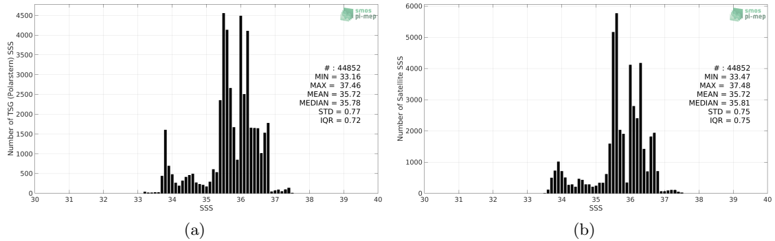
Figure 2: Histograms of SSS from TSG (Polarstern) (a) and Aquarius SSS L4 OI v5 - Weekly (IPRC) (b) considering all match-up pairs per bins of 0.1 over the South Atlantic Ocean Pi-MEP region and for the full satellite product period.
