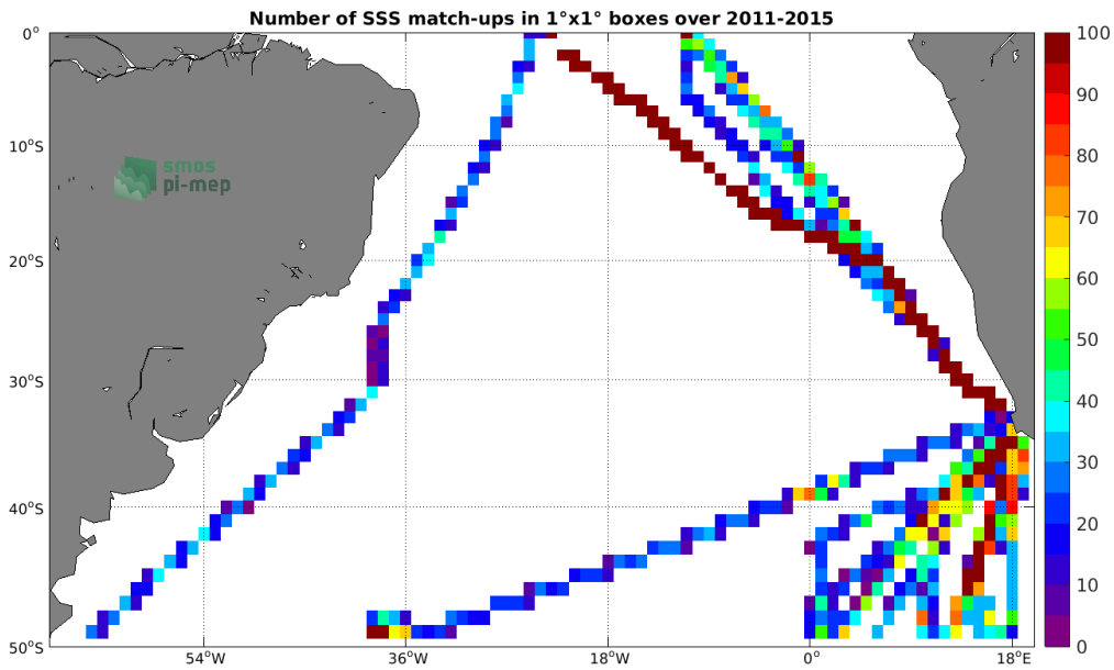
Figure 4: Number of SSS match-ups between TSG (Polarstern) SSS and the Aquarius SSS L4 OI v5 - Weekly (IPRC) SSS product for the South Atlantic Ocean Pi-MEP region over 1°x1° boxes and for the full satellite product period.
