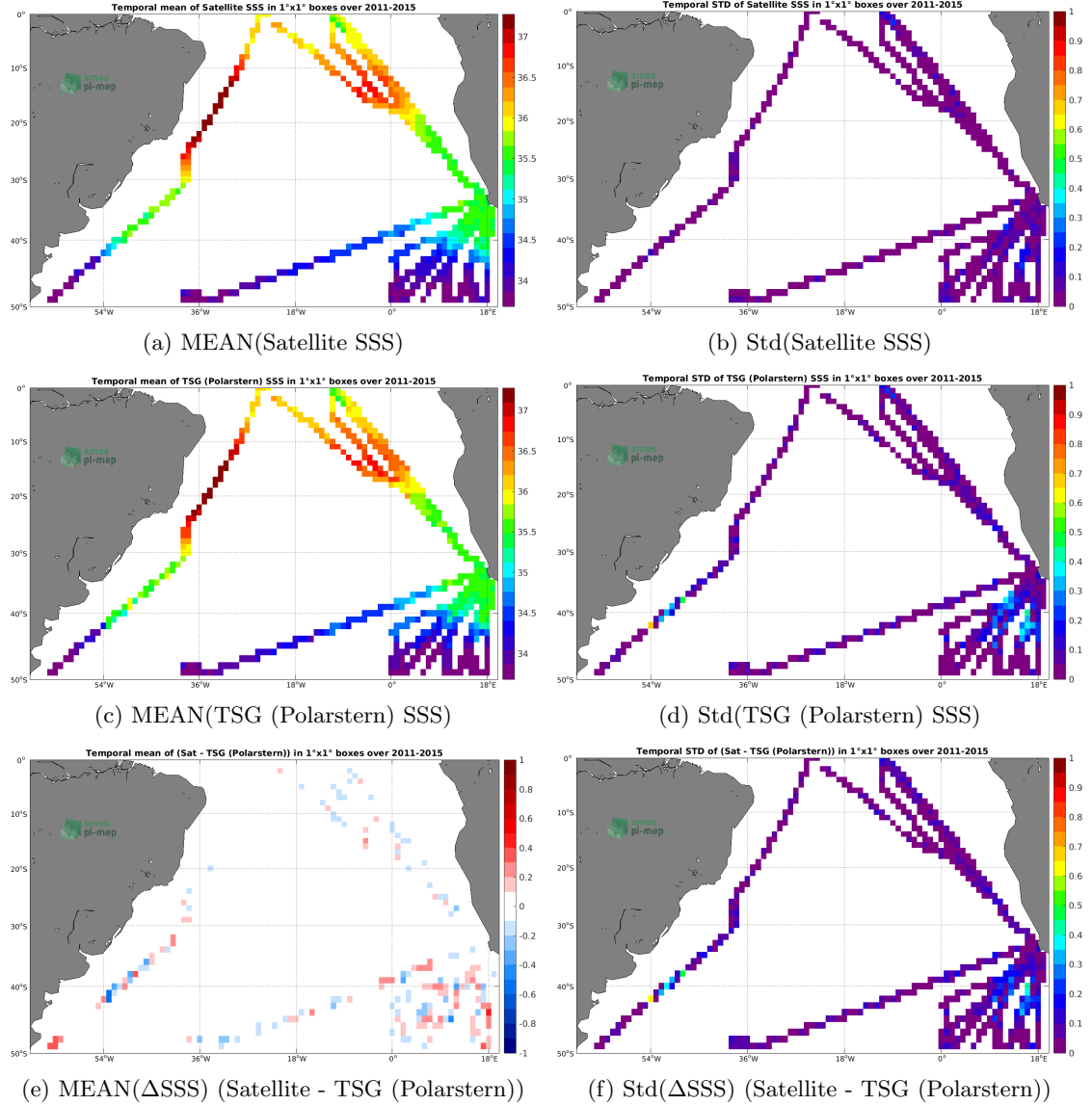
Figure 6: Temporal mean (left) and Std (right) of SSS from Aquarius SSS L4 OI v5 - Weekly (IPRC) (top), TSG (Polarstern) (middle), and of \Delta SSS (Satellite - TSG (Polarstern)). Only match-up pairs are used to generate these maps.
