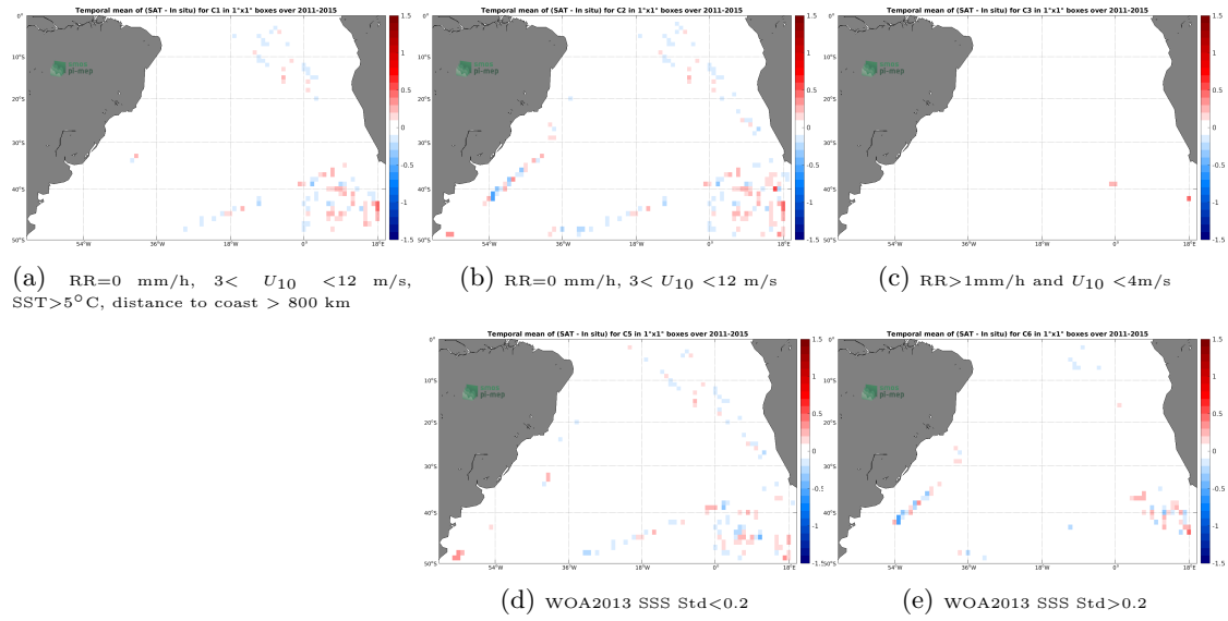
Figure 12: Temporal mean gridded over spatial boxes of size 1^\circ \times 1^\circ of \Delta SSS (Aquarius SSS L4 OI v5 - Weekly (IPRC) - TSG (Polarstern)) for 5 different subdatasets corresponding to: RR=0 mm/h, 3 < U_{10} < 12 m/s, SST > 5^\circ\text{C} , distance to coast > 800 km (a), RR=0 mm/h, 3 < U_{10} < 12 m/s (b), RR > 1 mm/h and U_{10} < 4 m/s (c), WOA2013 SSS Std < 0.2 (d), WOA2013 SSS Std > 0.2 (e).
