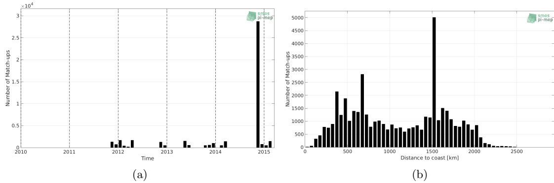
Figure 1: Number of match-ups between TSG-POLARSTERN and Aquarius-L4-IPRC-V5-WEEKLY SSS as a function of time (a) and as function of the distance to coast (b) over the South Atlantic Ocean Pi-MEP region and for the full satellite product period.
