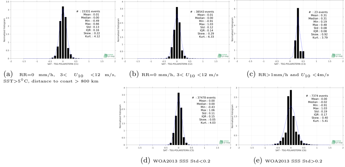
Figure 13: Normalized histogram of \Delta SSS (Aquarius-L4-IPRC-V5-WEEKLY - TSG-POLARSTERN) for 5 different subdatasets corresponding to: RR=0 mm/h, 3 < U_{10} < 12 m/s, SST > 5^\circ C , distance to coast > 800 km (a), RR=0 mm/h, 3 < U_{10} < 12 m/s (b), RR > 1 mm/h and U_{10} < 4 m/s (c), WOA2013 SSS Std < 0.2 (d), WOA2013 SSS Std > 0.2 (e).
