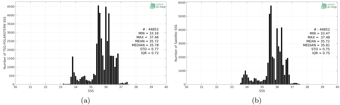
Figure 2: Histograms of SSS from TSG-POLARSTERN (a) and Aquarius-L4-IPRC-V5-WEEKLY (b) considering all match-up pairs per bins of 0.1 over the South Atlantic Ocean Pi-MEP region and for the full satellite product period.
