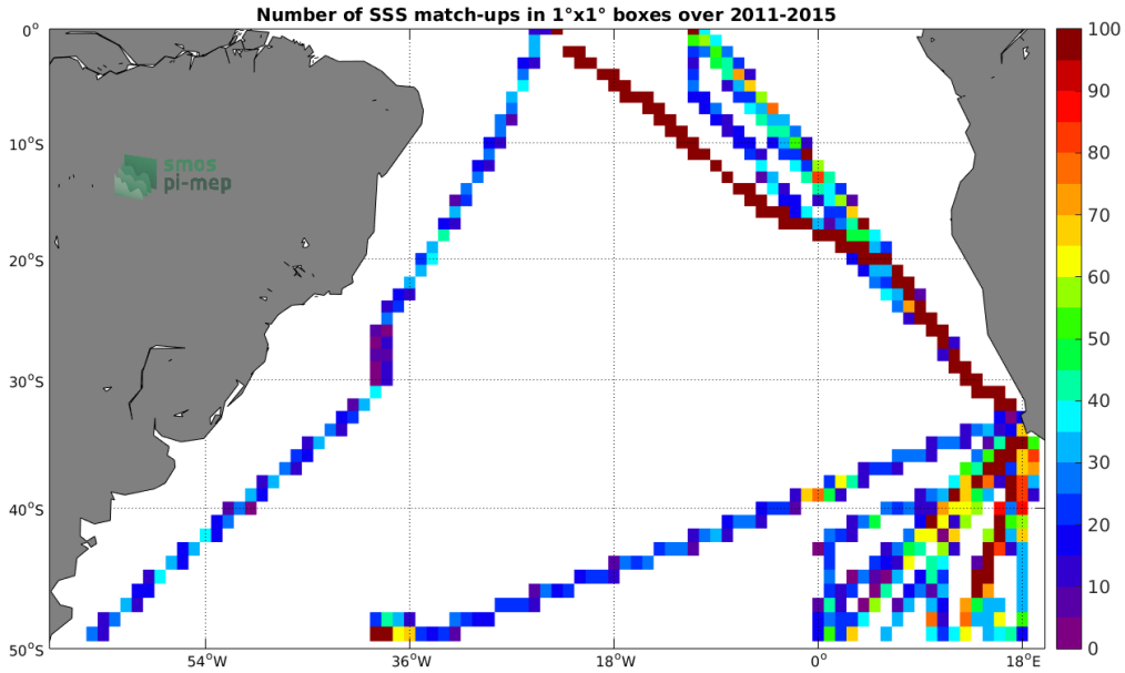
Figure 4: Number of SSS match-ups between TSG-POLARSTERN SSS and the Aquarius-L4-IPRC-V5-WEEKLY SSS product for the South Atlantic Ocean Pi-MEP region over 1°x1° boxes and for the full satellite product period.
