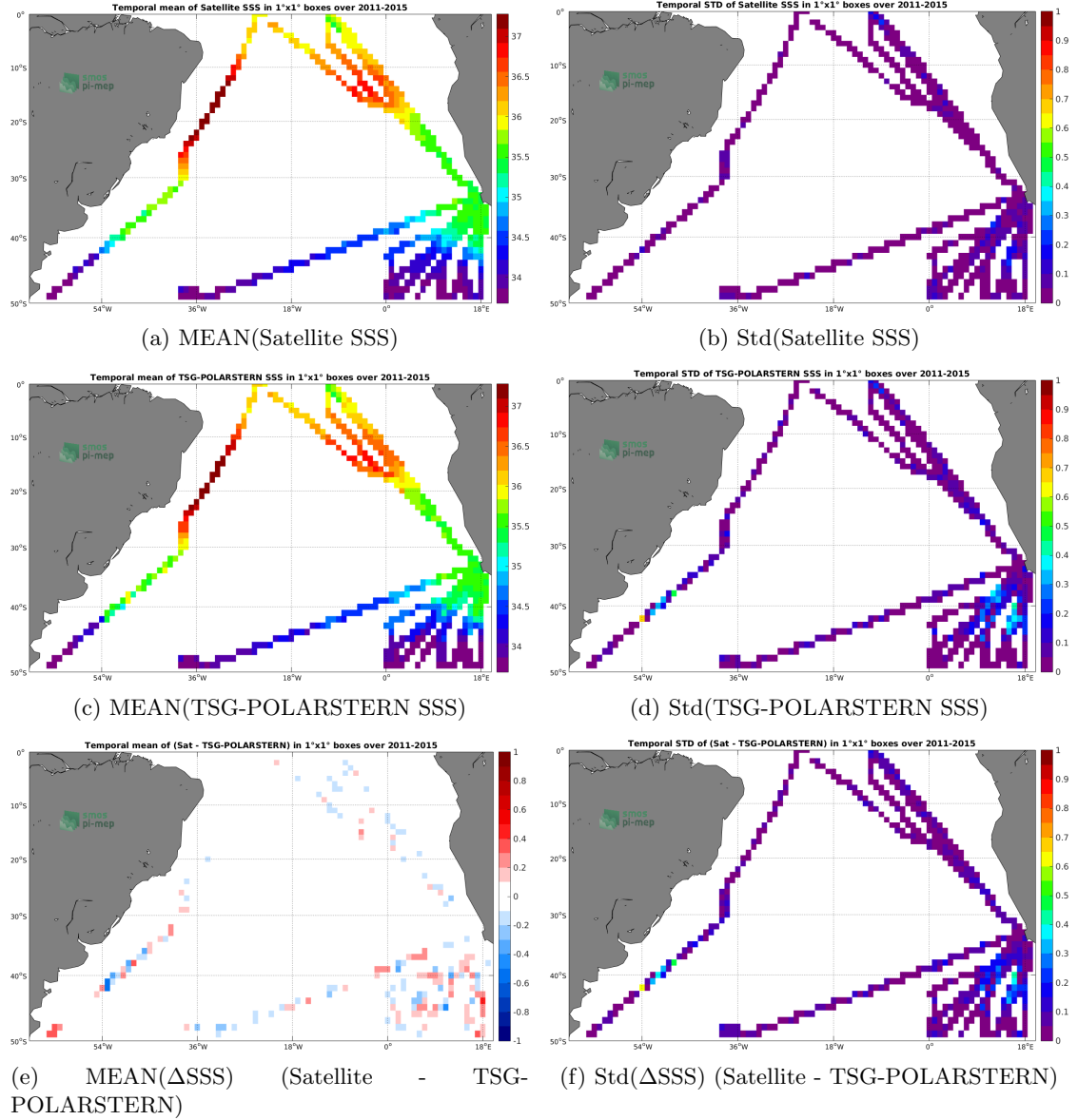
Figure 6: Temporal mean (left) and Std (right) of SSS from Aquarius-L4-IPRC-V5-WEEKLY (top), TSG-POLARSTERN (middle), and of \Delta SSS (Satellite - TSG-POLARSTERN). Only match-up pairs are used to generate these maps.
