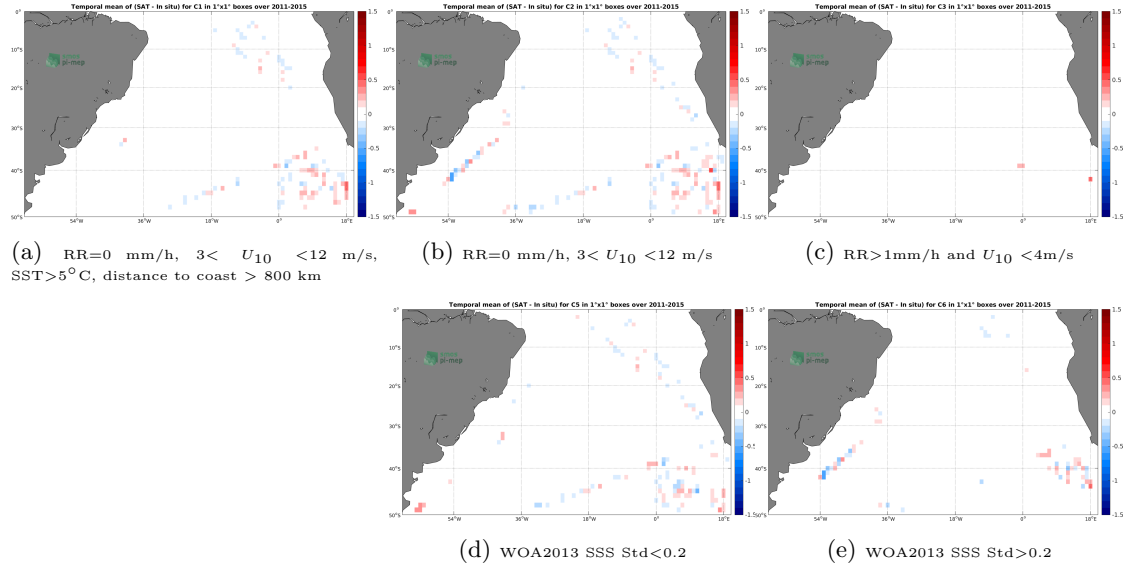
Figure 12: Temporal mean gridded over spatial boxes of size 1^\circ \times 1^\circ of \Delta SSS (Aquarius-L4-IPRC-V5-WEEKLY - TSG-POLARSTERN) for 5 different subdatasets corresponding to: RR=0 mm/h, 3 < U_{10} < 12 m/s, SST > 5^\circ C , distance to coast > 800 km (a), RR=0 mm/h, 3 < U_{10} < 12 m/s (b), RR > 1 mm/h and U_{10} < 4 m/s (c), WOA2013 SSS Std < 0.2 (d), WOA2013 SSS Std > 0.2 (e).
