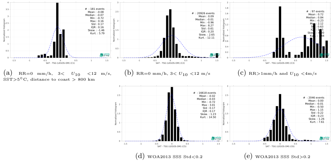
Figure 15: Normalized histogram of \Delta\text{SSS} (Aquarius SSS L4 OI v5 - Weekly (IPRC) - TSG (LEGOS-DM)) for 5 different subdatasets corresponding to: RR=0 mm/h, 3 < U_{10} < 12 m/s, SST>5°C, distance to coast > 800 km (a), RR=0 mm/h, 3 < U_{10} < 12 m/s (b), RR>1mm/h and U_{10} < 4 m/s (c), WOA2013 SSS Std<0.2 (d), WOA2013 SSS Std>0.2 (e).
