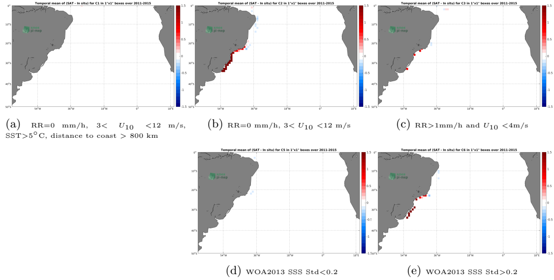
Figure 12: Temporal mean gridded over spatial boxes of size 1^\circ \times 1^\circ of \Delta SSS (Aquarius-L4-IPRC-V5-WEEKLY - TSG-LEGOS-DM) for 5 different subdatasets corresponding to: RR=0 mm/h, 3 < U_{10} < 12 m/s, SST > 5^\circ C , distance to coast > 800 km (a), RR=0 mm/h, 3 < U_{10} < 12 m/s (b), RR > 1 mm/h and U_{10} < 4 m/s (c), WOA2013 SSS Std < 0.2 (d), WOA2013 SSS Std > 0.2 (e).
