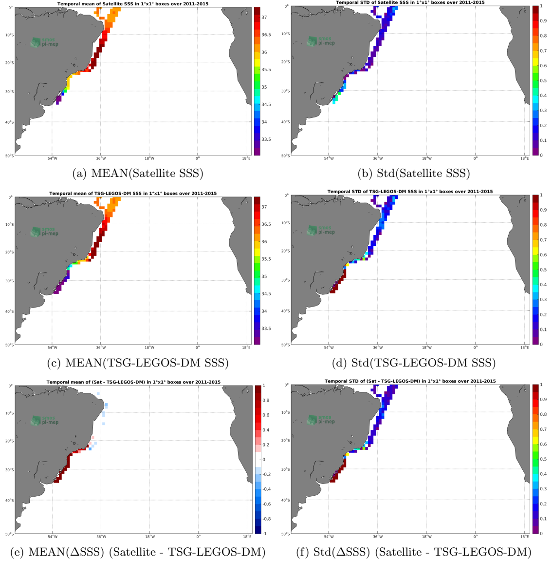
Figure 6: Temporal mean (left) and Std (right) of SSS from Aquarius-L4-IPRC-V5-WEEKLY (top), TSG-LEGOS-DM (middle), and of \Delta SSS (Satellite - TSG-LEGOS-DM). Only match-up pairs are used to generate these maps.
