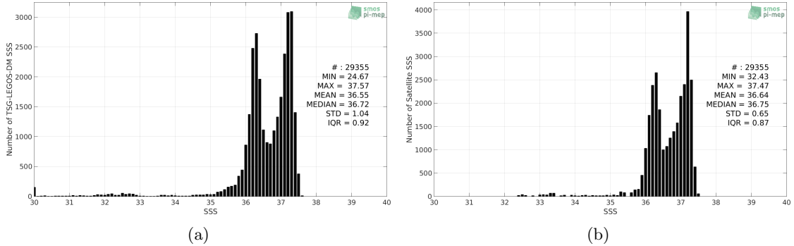
Figure 2: Histograms of SSS from TSG-LEGOS-DM (a) and Aquarius-L4-IPRC-V5-WEEKLY (b) considering all match-up pairs per bins of 0.1 over the South Atlantic Ocean Pi-MEP region and for the full satellite product period.
