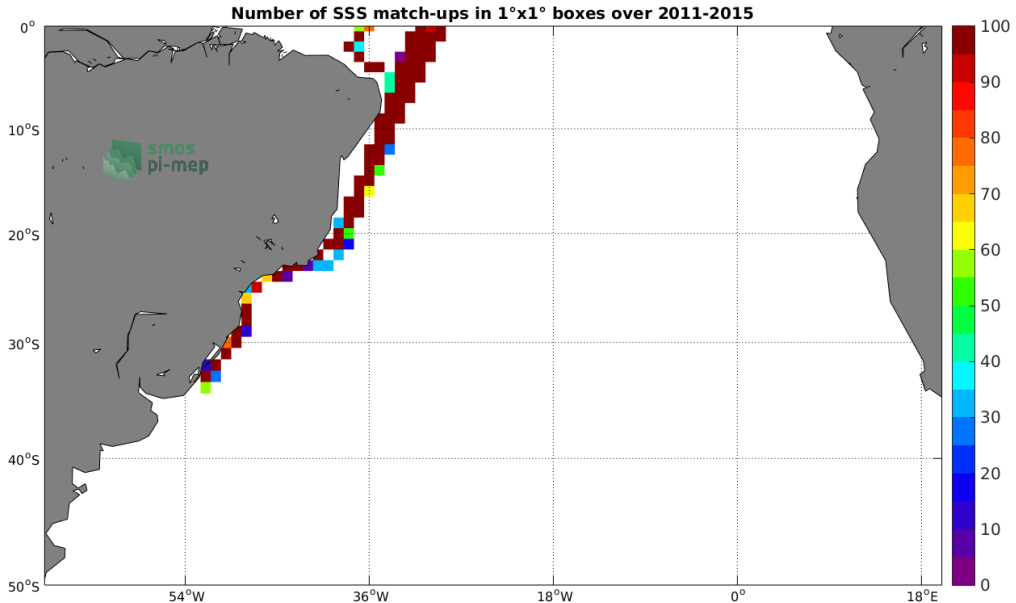
Figure 4: Number of SSS match-ups between TSG-LEGOS-DM SSS and the Aquarius-L4-IPRC-V5-WEEKLY SSS product for the South Atlantic Ocean Pi-MEP region over 1^\circ \times 1^\circ boxes and for the full satellite product period.
