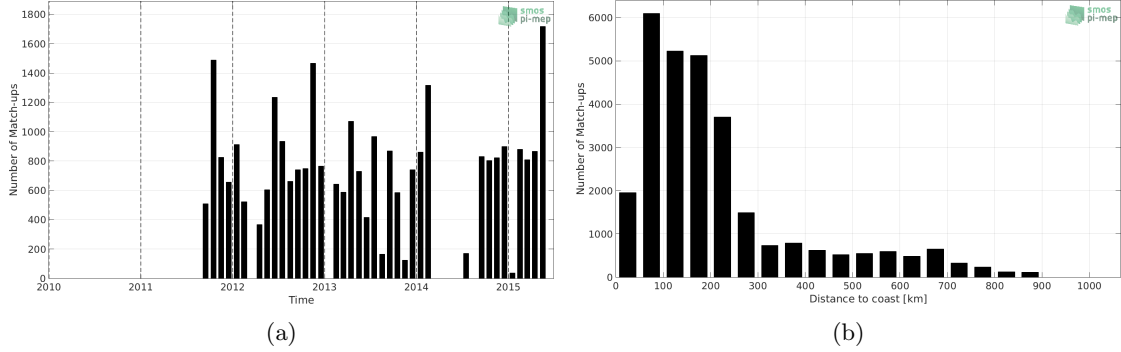
Figure 1: Number of match-ups between TSG-LEGOS-DM and Aquarius-L4-IPRC-V5-WEEKLY SSS as a function of time (a) and as function of the distance to coast (b) over the South Atlantic Ocean Pi-MEP region and for the full satellite product period.
