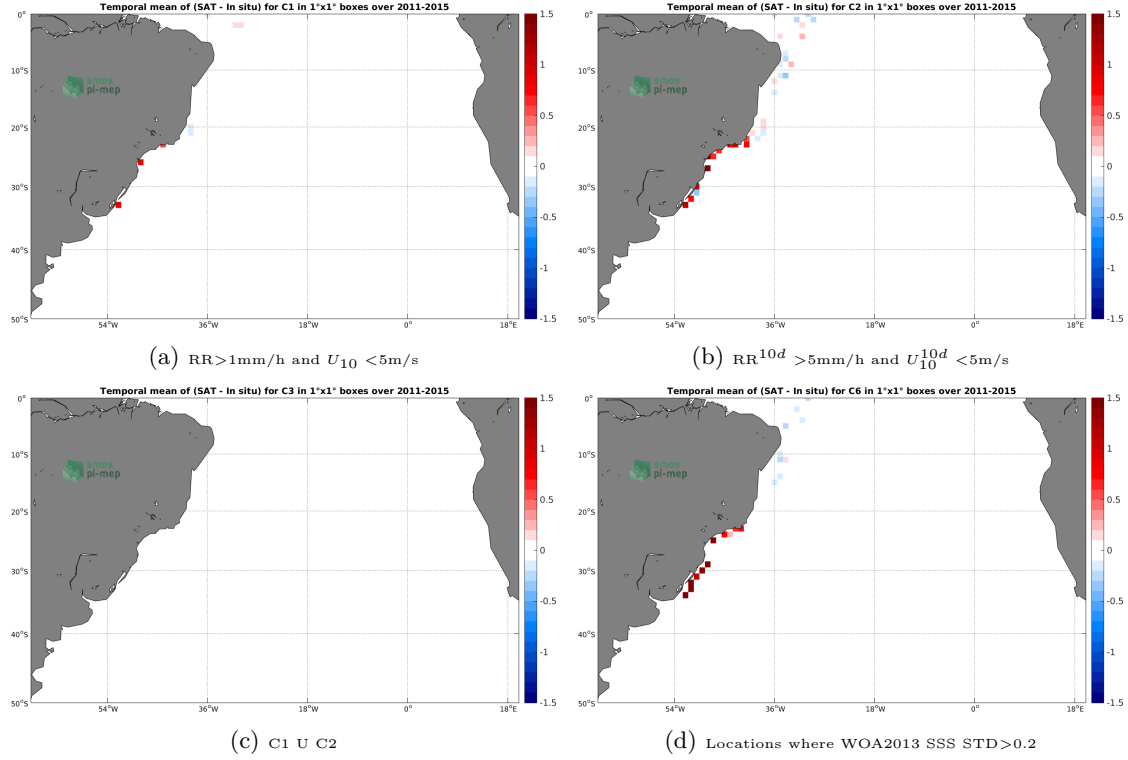
Figure 12: Temporal mean gridded over spatial boxes of size 1^\circ \times 1^\circ of \Delta SSS (Aquarius-L4-IPRC-V5-WEEKLY - TSG-LEGOS-DM) for 4 different subdatasets corresponding to: RR > 1mm/h and U_{10} < 5\text{m/s} (a), RR^{10d} > 5\text{mm/h} and U_{10}^{10d} < 5\text{m/s} (b), C1 U C2 (c), Locations where WOA2013 SSS STD > 0.2 (d).
