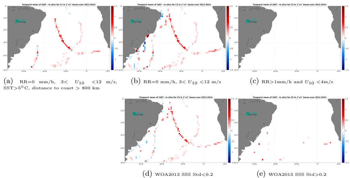
Figure 14: Temporal mean gridded over spatial boxes of size 1^\circ \times 1^\circ of \Delta SSS (Aquarius SSS L4 OI v5 - Weekly (IPRC) - TSG (GOSUD-Sailing-ship)) for 5 different subdatasets corresponding to:RR=0 mm/h, 3 < U_{10} < 12 m/s, SST >5^\circ\text{C} , distance to coast > 800 km (a), RR=0 mm/h, 3 < U_{10} < 12 m/s (b), RR >1 mm/h and U_{10} < 4 m/s (c), WOA2013 SSS Std <0.2 (d), WOA2013 SSS Std >0.2 (e).
