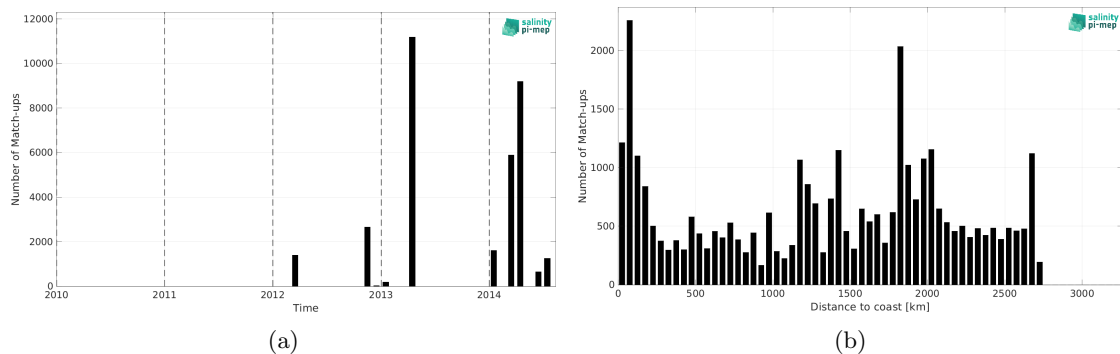
Figure 2: Number of match-ups between TSG (GOSUD-Sailing-ship) and Aquarius SSS L4 OI v5 - Weekly (IPRC) SSS as a function of time (a) and as function of the distance to coast (b) over the South Atlantic Ocean Pi-MEP region and for the full satellite product period.
