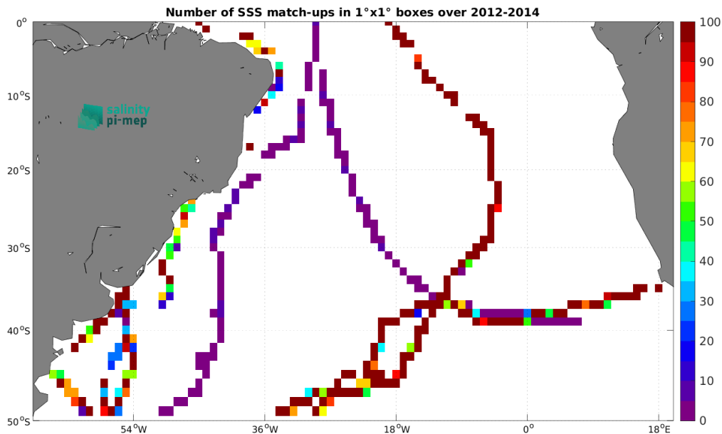
Figure 5: Number of SSS match-ups between TSG (GOSUD-Sailing-ship) SSS and the Aquarius SSS L4 OI v5 - Weekly (IPRC) SSS product for the South Atlantic Ocean Pi-MEP region over 1^\circ \times 1^\circ boxes and for the full satellite product period.
