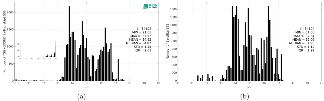
Figure 3: Histograms of SSS from TSG (GOSUD-Sailing-ship) (a) and Aquarius SSS L4 OI v5 - Weekly (IPRC) (b) considering all match-up pairs per bins of 0.1 over the South Atlantic Ocean Pi-MEP region and for the full satellite product period.
