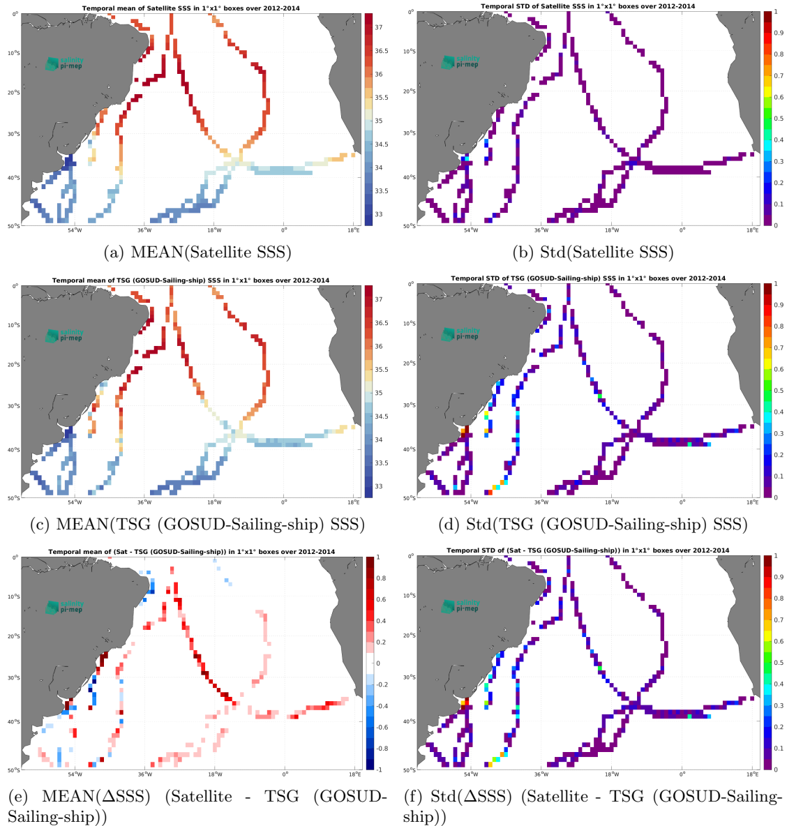
Figure 7: Temporal mean (left) and Std (right) of SSS from Aquarius SSS L4 OI v5 - Weekly (IPRC) (top), TSG (GOSUD-Sailing-ship) (middle), and of \Delta SSS (Satellite - TSG (GOSUD-Sailing-ship)). Only match-up pairs are used to generate these maps.
