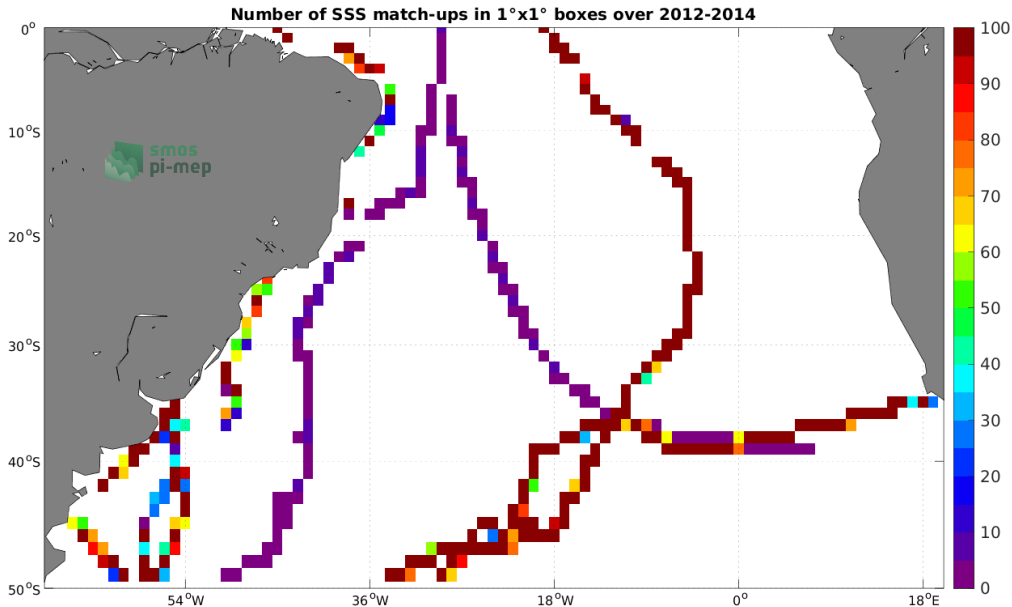
Figure 4: Number of SSS match-ups between TSG (GOSUD-Sailing-ship) SSS and the Aquarius SSS L4 OI v5 - Weekly (IPRC) SSS product for the South Atlantic Ocean Pi-MEP region over 1^\circ \times 1^\circ boxes and for the full satellite product period.
