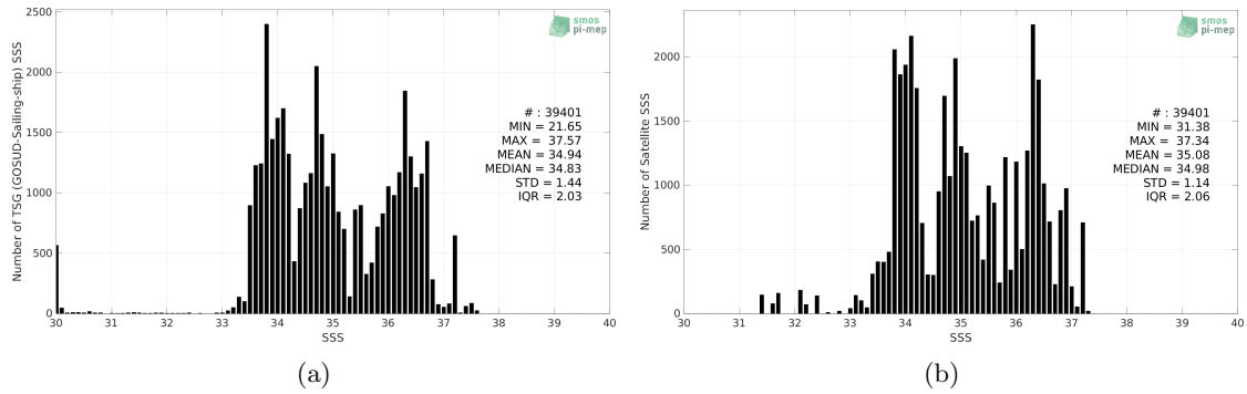
Figure 2: Histograms of SSS from TSG (GOSUD-Sailing-ship) (a) and Aquarius SSS L4 OI v5 - Weekly (IPRC) (b) considering all match-up pairs per bins of 0.1 over the South Atlantic Ocean Pi-MEP region and for the full satellite product period.
