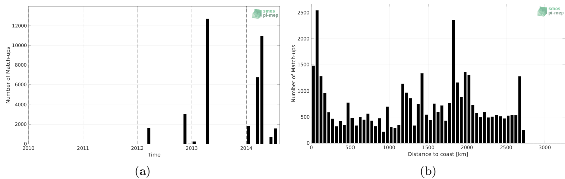
Figure 1: Number of match-ups between TSG (GOSUD-Sailing-ship) and Aquarius SSS L4 OI v5 - Weekly (IPRC) SSS as a function of time (a) and as function of the distance to coast (b) over the South Atlantic Ocean Pi-MEP region and for the full satellite product period.
