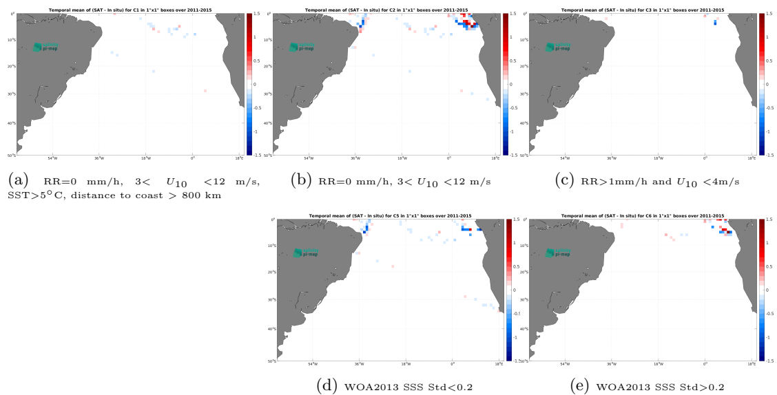
Figure 14: Temporal mean gridded over spatial boxes of size 1^\circ \times 1^\circ of \Delta\text{SSS} (Aquarius SSS L4 OI v5 - Weekly (IPRC) - TSG (GOSUD-Research-vessel)) for 5 different subdatasets corresponding to:RR=0 mm/h, 3 < U_{10} < 12 m/s, SST >5^\circ\text{C} , distance to coast > 800 km (a), RR=0 mm/h, 3 < U_{10} < 12 m/s (b), RR >1 mm/h and U_{10} < 4 m/s (c), WOA2013 SSS Std <0.2 (d), WOA2013 SSS Std >0.2 (e).
