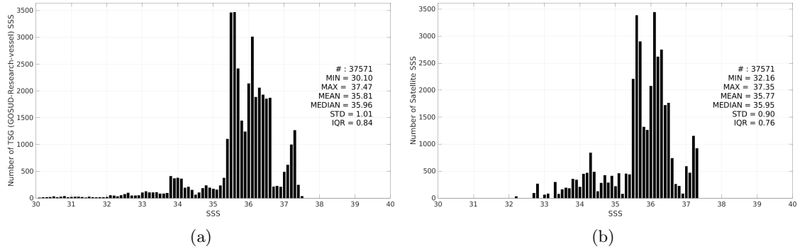
Figure 3: Histograms of SSS from TSG (GOSUD-Research-vessel) (a) and Aquarius SSS L4 OI v5 - Weekly (IPRC) (b) considering all match-up pairs per bins of 0.1 over the South Atlantic Ocean Pi-MEP region and for the full satellite product period.
