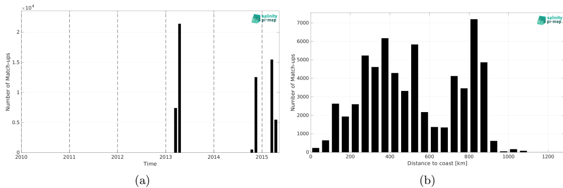
Figure 2: Number of match-ups between TSG (CSIC-UTM) and Aquarius SSS L4 OI v5 - Weekly (IPRC) SSS as a function of time (a) and as function of the distance to coast (b) over the South Atlantic Ocean Pi-MEP region and for the full satellite product period.
