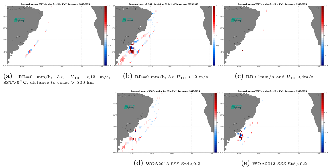
Figure 14: Temporal mean gridded over spatial boxes of size 1^\circ \times 1^\circ of \Delta\text{SSS} (Aquarius SSS L4 OI v5 - Weekly (IPRC) - TSG (CSIC-UTM)) for 5 different subdatasets corresponding to:RR=0 mm/h, 3 < U_{10} < 12 m/s, SST >5^\circ\text{C} , distance to coast > 800 km (a), RR=0 mm/h, 3 < U_{10} < 12 m/s (b), RR >1 mm/h and U_{10} < 4 m/s (c), WOA2013 SSS Std <0.2 (d), WOA2013 SSS Std >0.2 (e).
