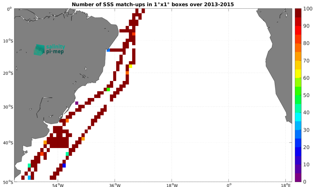
Figure 5: Number of SSS match-ups between TSG (CSIC-UTM) SSS and the Aquarius SSS L4 OI v5 - Weekly (IPRC) SSS product for the South Atlantic Ocean Pi-MEP region over 1^\circ \times 1^\circ boxes and for the full satellite product period.
