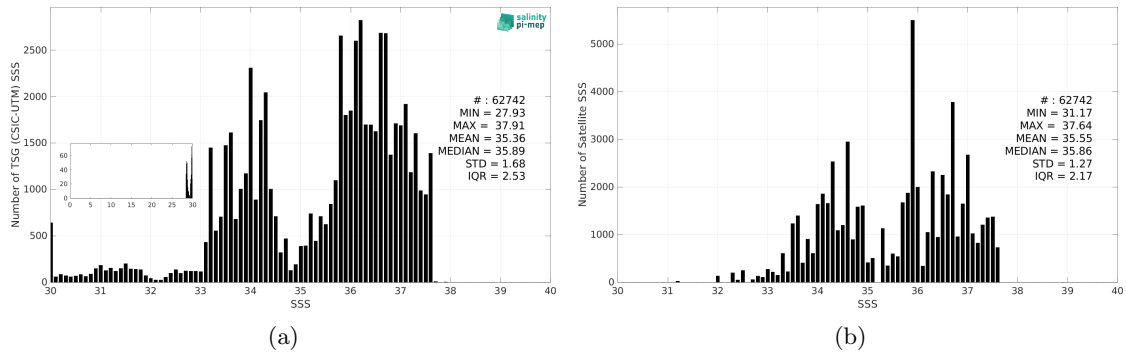
Figure 3: Histograms of SSS from TSG (CSIC-UTM) (a) and Aquarius SSS L4 OI v5 - Weekly (IPRC) (b) considering all match-up pairs per bins of 0.1 over the South Atlantic Ocean Pi-MEP region and for the full satellite product period.
