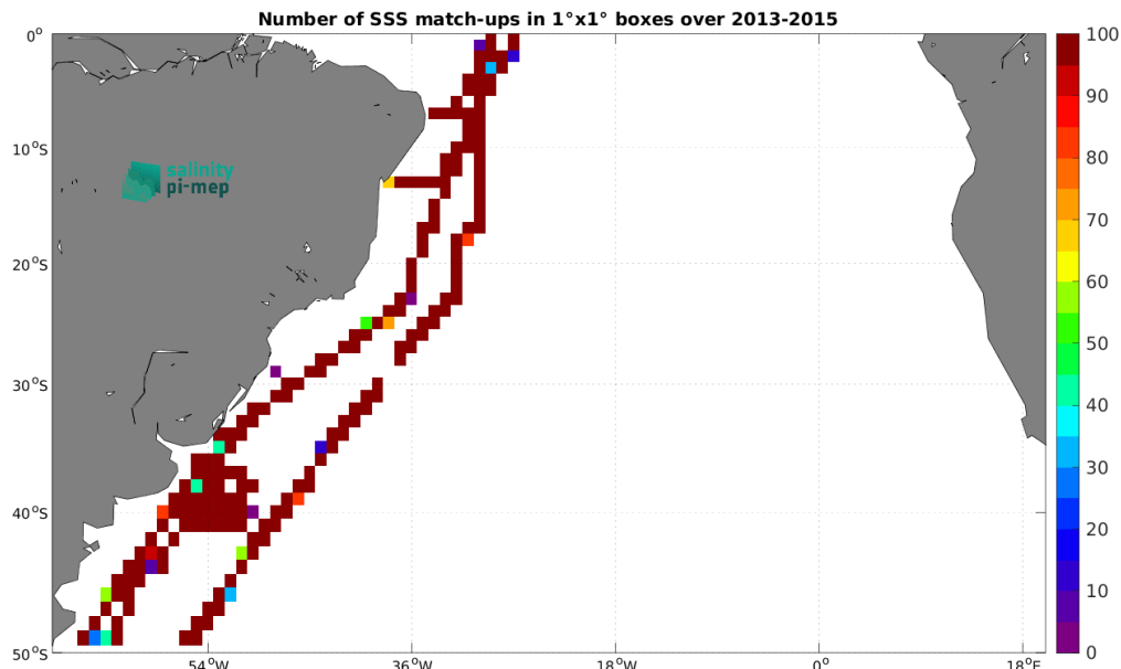
Figure 4: Number of SSS match-ups between TSG (CSIC-UTM) SSS and the Aquarius SSS L4 OI v5 - Weekly (IPRC) SSS product for the South Atlantic Ocean Pi-MEP region over 1^\circ \times 1^\circ boxes and for the full satellite product period.
