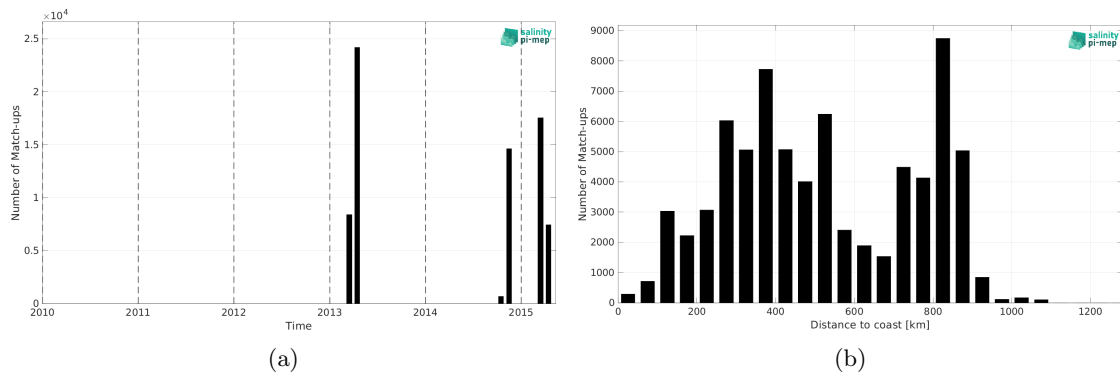
Figure 1: Number of match-ups between TSG (CSIC-UTM) and Aquarius SSS L4 OI v5 - Weekly (IPRC) SSS as a function of time (a) and as function of the distance to coast (b) over the South Atlantic Ocean Pi-MEP region and for the full satellite product period.
