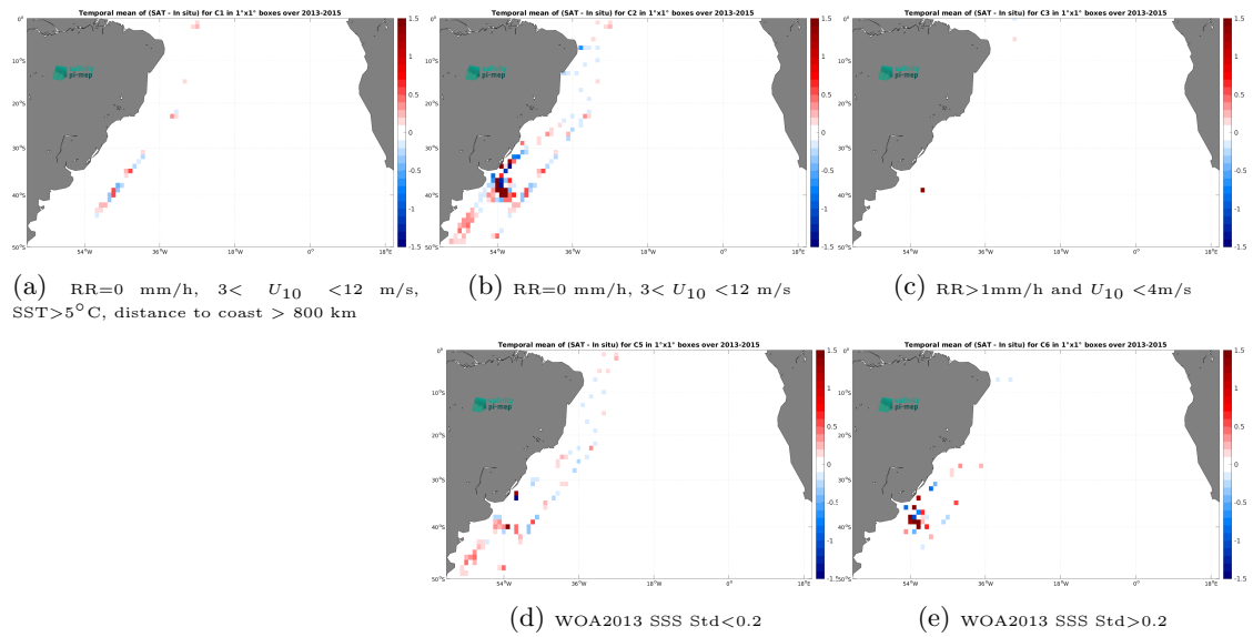
Figure 12: Temporal mean gridded over spatial boxes of size 1^\circ \times 1^\circ of \Delta SSS (Aquarius SSS L4 OI v5 - Weekly (IPRC) - TSG (CSIC-UTM)) for 5 different subdatasets corresponding to:RR=0 mm/h, 3 < U_{10} < 12 m/s, SST >5^\circ\text{C} , distance to coast > 800 km (a), RR=0 mm/h, 3 < U_{10} < 12 m/s (b), RR >1 mm/h and U_{10} < 4 m/s (c), WOA2013 SSS Std <0.2 (d), WOA2013 SSS Std >0.2 (e).
