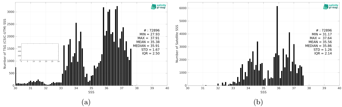
Figure 2: Histograms of SSS from TSG (CSIC-UTM) (a) and Aquarius SSS L4 OI v5 - Weekly (IPRC) (b) considering all match-up pairs per bins of 0.1 over the South Atlantic Ocean Pi-MEP region and for the full satellite product period.
