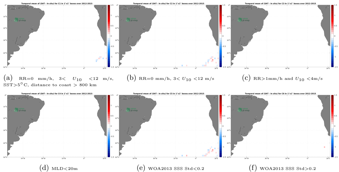
Figure 12: Temporal mean gridded over spatial boxes of size 1^{\circ}\times 1^{\circ} of \Delta\text{SSS} (Aquarius SSS L4 OI v5 - Weekly (IPRC) - Marine mammals) for 6 different subdatasets corresponding to:RR=0 mm/h, 3 < U_{10} < 12 m/s, SST > 5^{\circ}\text{C} , distance to coast > 800 km (a), RR=0 mm/h, 3 < U_{10} < 12 m/s (b), RR > 1\text{mm/h} and U_{10} < 4\text{m/s} (c),MLD < 20\text{m} (d),WOA2013 SSS Std < 0.2 (e),WOA2013 SSS Std > 0.2 (f).
