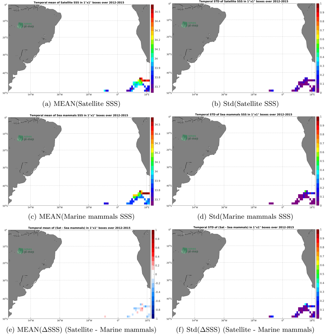
Figure 6: Temporal mean (left) and Std (right) of SSS from Aquarius SSS L4 OI v5 - Weekly (IPRC) (top), Marine mammals (middle), and of \Delta SSS (Satellite - Marine mammals). Only match-up pairs are used to generate these maps.
