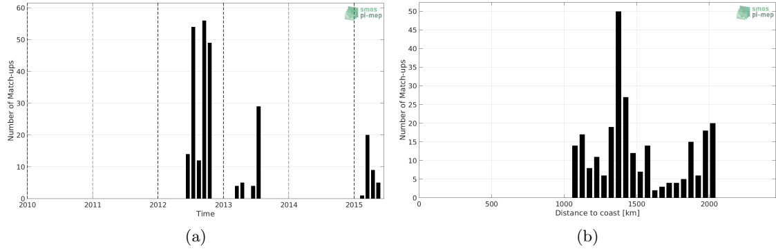
Figure 1: Number of match-ups between Marine mammals and Aquarius SSS L4 OI v5 - Weekly (IPRC) SSS as a function of time (a) and as function of the distance to coast (b) over the South Atlantic Ocean Pi-MEP region and for the full satellite product period.
