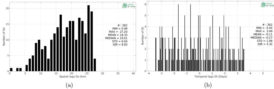
Figure 5: Histograms of the spatial (a) and temporal (b) lags between the location/time of the Marine mammals measurement and the date of the corresponding Aquarius SSS L4 OI v5 - Weekly (IPRC) SSS pixel.
