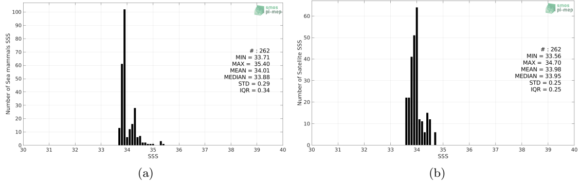
Figure 2: Histograms of SSS from Marine mammals (a) and Aquarius SSS L4 OI v5 - Weekly (IPRC) (b) considering all match-up pairs per bins of 0.1 over the South Atlantic Ocean Pi-MEP region and for the full satellite product period.
