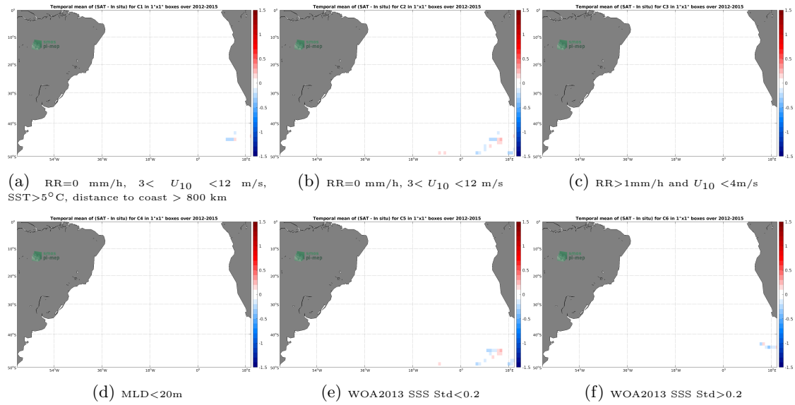
Figure 12: Temporal mean gridded over spatial boxes of size 1^{\circ} \times 1^{\circ} of \Delta\text{SSS} (Aquarius SSS L4 OI v5 - Weekly (IPRC) - Marine mammals) for 6 different subdatasets corresponding to: \text{RR}=0 mm/h, 3 < U_{10} < 12 m/s, SST > 5^{\circ}\text{C} , distance to coast > 800 km (a), \text{RR}=0 mm/h, 3 < U_{10} < 12 m/s (b), \text{RR} > 1\text{mm/h} and U_{10} < 4\text{m/s} (c), \text{MLD} < 20\text{m} (d), WOA2013 SSS Std < 0.2 (e), WOA2013 SSS Std > 0.2 (f).
