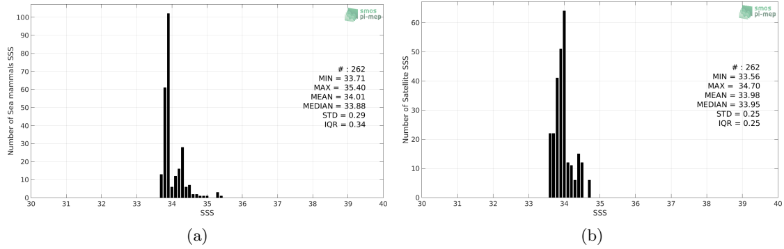
Figure 2: Histograms of SSS from Sea mammals (a) and Aquarius-L4-IPRC-V5-WEEKLY (b) considering all match-up pairs per bins of 0.1 over the South Atlantic Ocean Pi-MEP region and for the full satellite product period.
