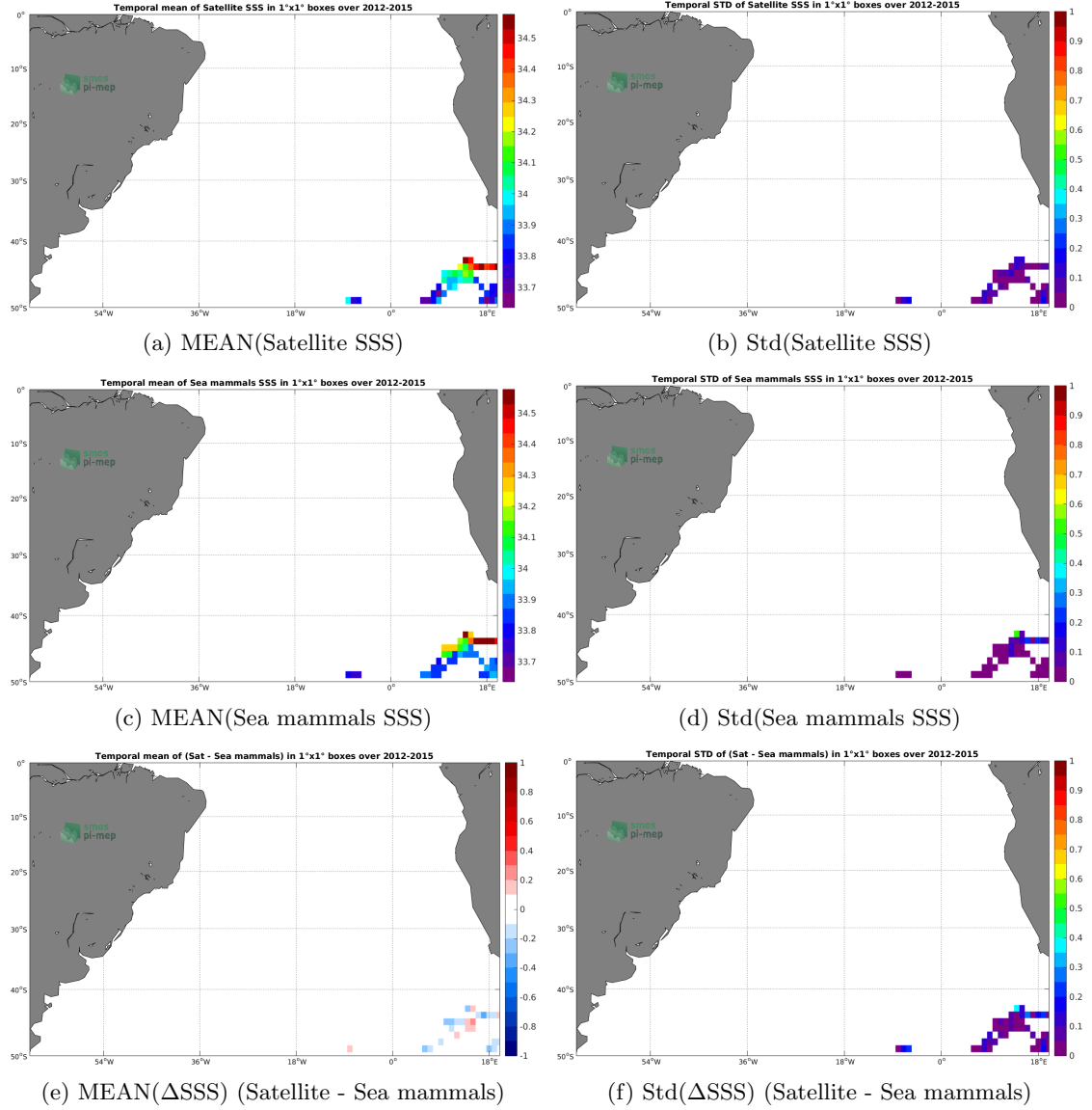
Figure 6: Temporal mean (left) and Std (right) of SSS from Aquarius-L4-IPRC-V5-WEEKLY (top), Sea mammals (middle), and of \Delta SSS (Satellite - Sea mammals). Only match-up pairs are used to generate these maps.
