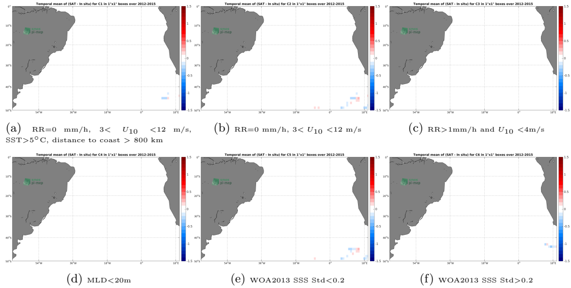
Figure 12: Temporal mean gridded over spatial boxes of size 1^{\circ}\times 1^{\circ} of \Delta\text{SSS} (Aquarius-L4-IPRC-V5-WEEKLY - Sea mammals) for 6 different subdatasets corresponding to: \text{RR}=0 mm/h, 3 < U_{10} < 12 m/s, SST > 5^{\circ}\text{C} , distance to coast > 800 km (a), \text{RR}=0 mm/h, 3 < U_{10} < 12 m/s (b), \text{RR} > 1\text{mm/h} and U_{10} < 4\text{m/s} (c), \text{MLD} < 20\text{m} (d), WOA2013 SSS Std < 0.2 (e), WOA2013 SSS Std > 0.2 (f).
