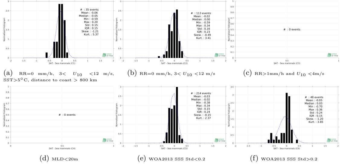
Figure 13: Normalized histogram of \Delta\text{SSS} (Aquarius-L4-IPRC-V5-WEEKLY - Sea mammals) for 6 different subdatasets corresponding to: RR=0 mm/h, 3 < U_{10} < 12 m/s, SST > 5^\circ\text{C} , distance to coast > 800 km (a), RR=0 mm/h, 3 < U_{10} < 12 m/s (b), RR > 1 mm/h and U_{10} < 4 m/s (c), MLD < 20 m (d), WOA2013 SSS Std < 0.2 (e), WOA2013 SSS Std > 0.2 (f).
