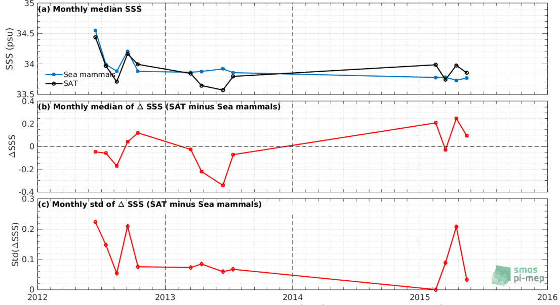
Figure 7: Time series of the monthly median SSS (top), median of \Delta\text{SSS} (Satellite - Sea mammals) and Std of \Delta\text{SSS} (Satellite - Sea mammals) over the South Atlantic Ocean Pi-MEP region considering all match-ups collected by the Pi-MEP.
