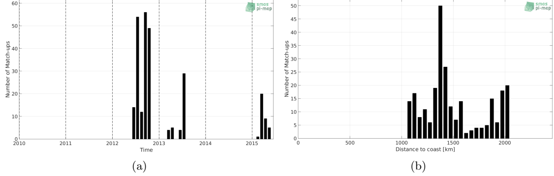
Figure 1: Number of match-ups between Sea mammals and Aquarius-L4-IPRC-V5-WEEKLY SSS as a function of time (a) and as function of the distance to coast (b) over the South Atlantic Ocean Pi-MEP region and for the full satellite product period.
