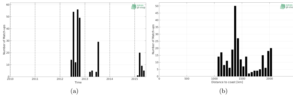
Figure 1: Number of match-ups between Sea mammals and Aquarius-L4-IPRC-V5-WEEKLY SSS as a function of time (a) and as function of the distance to coast (b) over the South Atlantic Ocean Pi-MEP region and for the full satellite product period.
