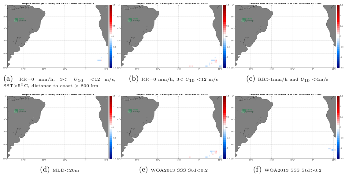
Figure 12: Temporal mean gridded over spatial boxes of size 1^\circ \times 1^\circ of \Delta SSS (Aquarius-L4-IPRC-V5-WEEKLY - Sea mammals) for 6 different subdatasets corresponding to:RR=0 mm/h, 3 < U_{10} < 12 m/s, SST >5^\circ C, distance to coast > 800 km (a), RR=0 mm/h, 3 < U_{10} < 12 m/s (b), RR >1 mm/h and U_{10} < 4 m/s (c),MLD <20 m (d),WOA2013 SSS Std <0.2 (e),WOA2013 SSS Std >0.2 (f).
