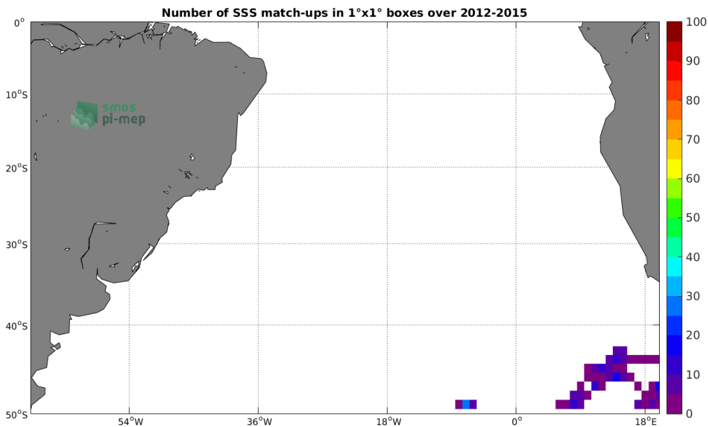
Figure 4: Number of SSS match-ups between Sea mammals SSS and the Aquarius-L4-IPRC-V5-WEEKLY SSS product for the South Atlantic Ocean Pi-MEP region over 1^\circ \times 1^\circ boxes and for the full satellite product period.
