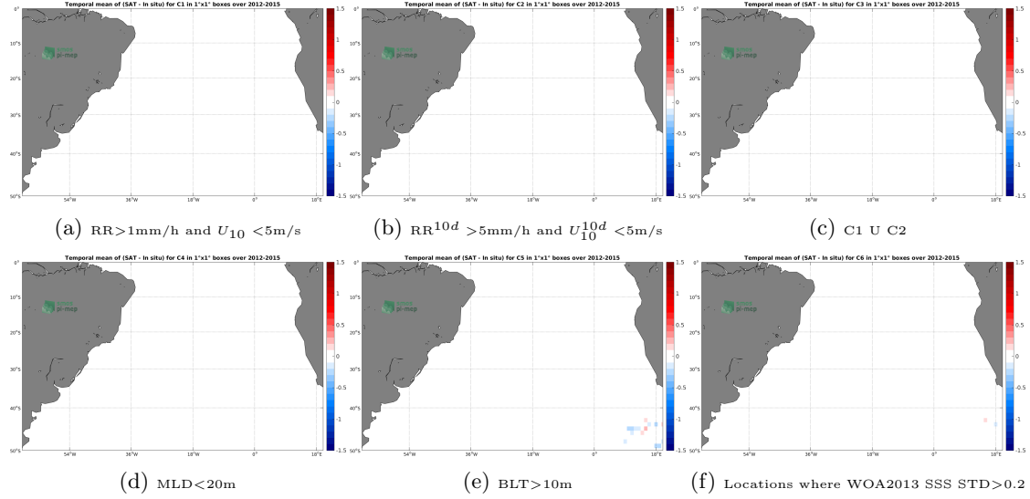
Figure 12: Temporal mean gridded over spatial boxes of size 1^\circ \times 1^\circ of \Delta\text{SSS} (Aquarius-L4-IPRC-V5-WEEKLY - Sea mammals) for 6 different subdatasets corresponding to: \text{RR} > 1\text{mm/h} and U_{10} < 5\text{m/s} (a), \text{RR}^{10d} > 5\text{mm/h} and U_{10}^{10d} < 5\text{m/s} (b), C1 U C2 (c), \text{MLD} < 20\text{m} (d), \text{BLT} > 10\text{m} (e), Locations where WOA2013 SSS STD > 0.2 (f).
