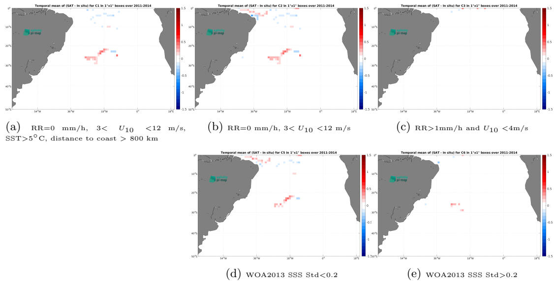
Figure 13: Temporal mean gridded over spatial boxes of size 1^\circ \times 1^\circ of \Delta\text{SSS} (Aquarius SSS L4 OI v5 - Weekly (IPRC) - Surface drifters) for 5 different subdatasets corresponding to:RR=0 mm/h, 3 < U_{10} < 12 m/s, SST >5^\circ\text{C} , distance to coast > 800 km (a), RR=0 mm/h, 3 < U_{10} < 12 m/s (b), RR >1 mm/h and U_{10} < 4 m/s (c), WOA2013 SSS Std <0.2 (d), WOA2013 SSS Std >0.2 (e).
