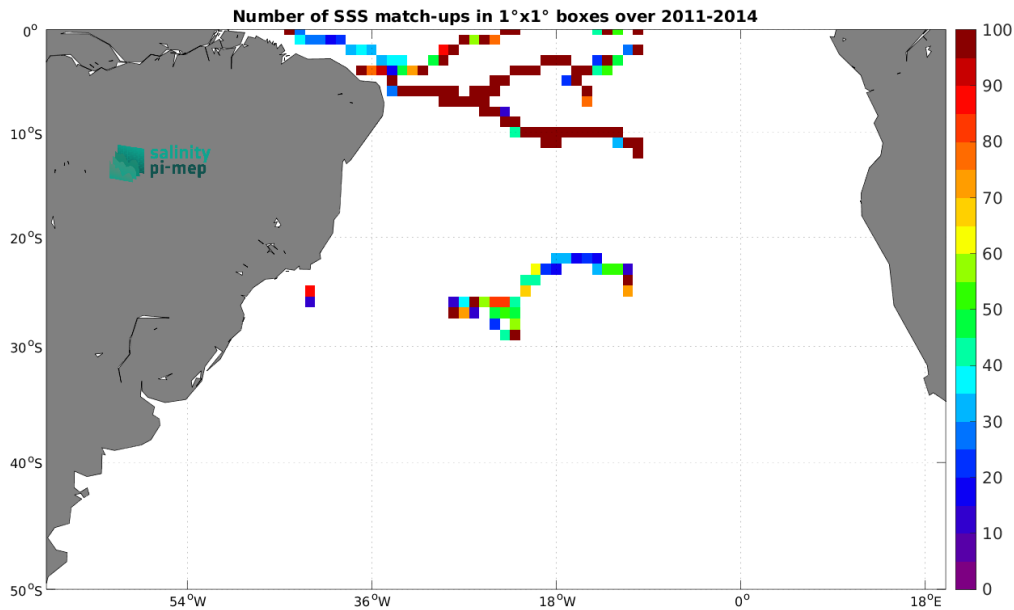
Figure 4: Number of SSS match-ups between Surface drifters SSS and the Aquarius SSS L4 OI v5 - Weekly (IPRC) SSS product for the South Atlantic Ocean Pi-MEP region over 1^\circ \times 1^\circ boxes and for the full satellite product period.
