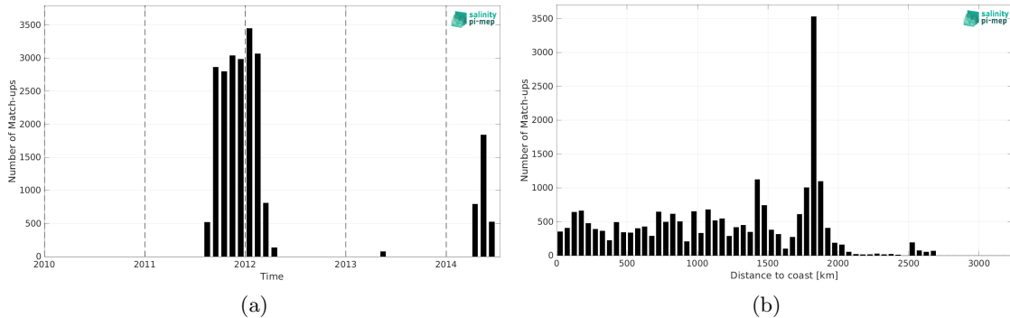
Figure 2: Number of match-ups between Surface drifters and Aquarius SSS L4 OI v5 - Weekly (IPRC) SSS as a function of time (a) and as function of the distance to coast (b) over the South Atlantic Ocean Pi-MEP region and for the full satellite product period.
