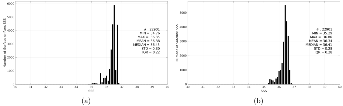
Figure 3: Histograms of SSS from Surface drifters (a) and Aquarius SSS L4 OI v5 - Weekly (IPRC) (b) considering all match-up pairs per bins of 0.1 over the South Atlantic Ocean Pi-MEP region and for the full satellite product period.
