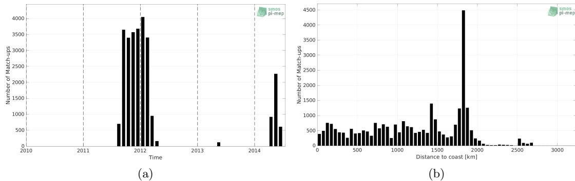
Figure 1: Number of match-ups between Surface drifters and Aquarius SSS L4 OI v5 - Weekly (IPRC) SSS as a function of time (a) and as function of the distance to coast (b) over the South Atlantic Ocean Pi-MEP region and for the full satellite product period.
