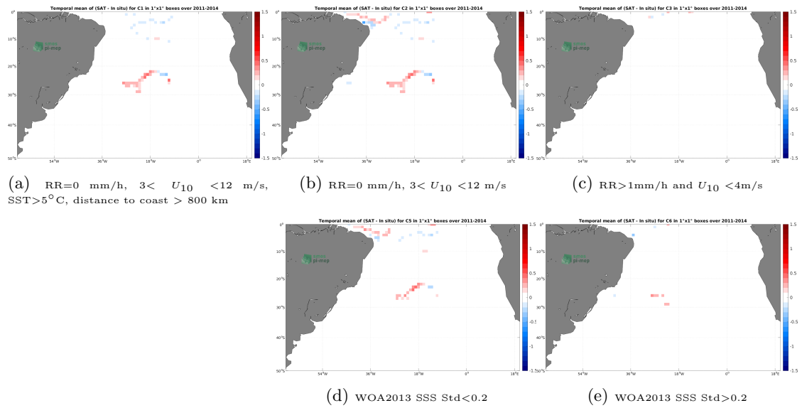
Figure 11: Temporal mean gridded over spatial boxes of size 1^\circ \times 1^\circ of \Delta SSS (Aquarius SSS L4 OI v5 - Weekly (IPRC) - Surface drifters) for 5 different subdatasets corresponding to:RR=0 mm/h, 3 < U_{10} < 12 m/s, SST >5^\circ\text{C} , distance to coast > 800 km (a), RR=0 mm/h, 3 < U_{10} < 12 m/s (b), RR >1 mm/h and U_{10} < 4 m/s (c), WOA2013 SSS Std <0.2 (d), WOA2013 SSS Std >0.2 (e).
