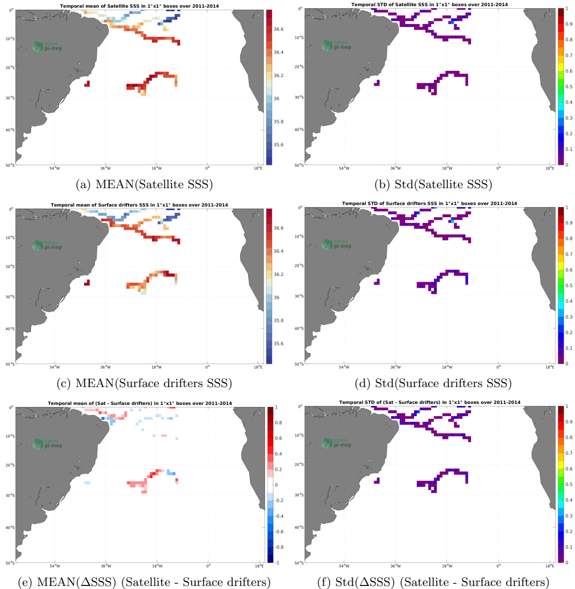
Figure 5: Temporal mean (left) and Std (right) of SSS from Aquarius SSS L4 OI v5 - Weekly (IPRC) (top), Surface drifters (middle), and of \Delta SSS (Satellite - Surface drifters). Only match-up pairs are used to generate these maps.
