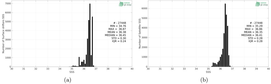
Figure 2: Histograms of SSS from Surface drifters (a) and Aquarius SSS L4 OI v5 - Weekly (IPRC) (b) considering all match-up pairs per bins of 0.1 over the South Atlantic Ocean Pi-MEP region and for the full satellite product period.
