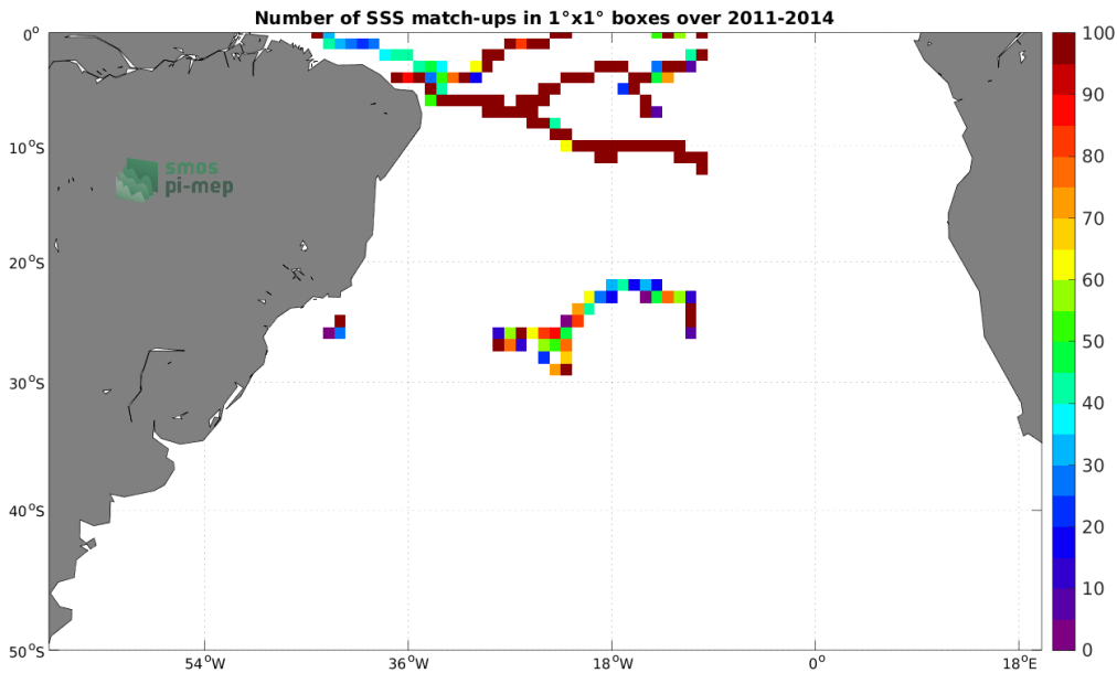
Figure 3: Number of SSS match-ups between Surface drifters SSS and the Aquarius SSS L4 OI v5 - Weekly (IPRC) SSS product for the South Atlantic Ocean Pi-MEP region over 1^\circ \times 1^\circ boxes and for the full satellite product period.
