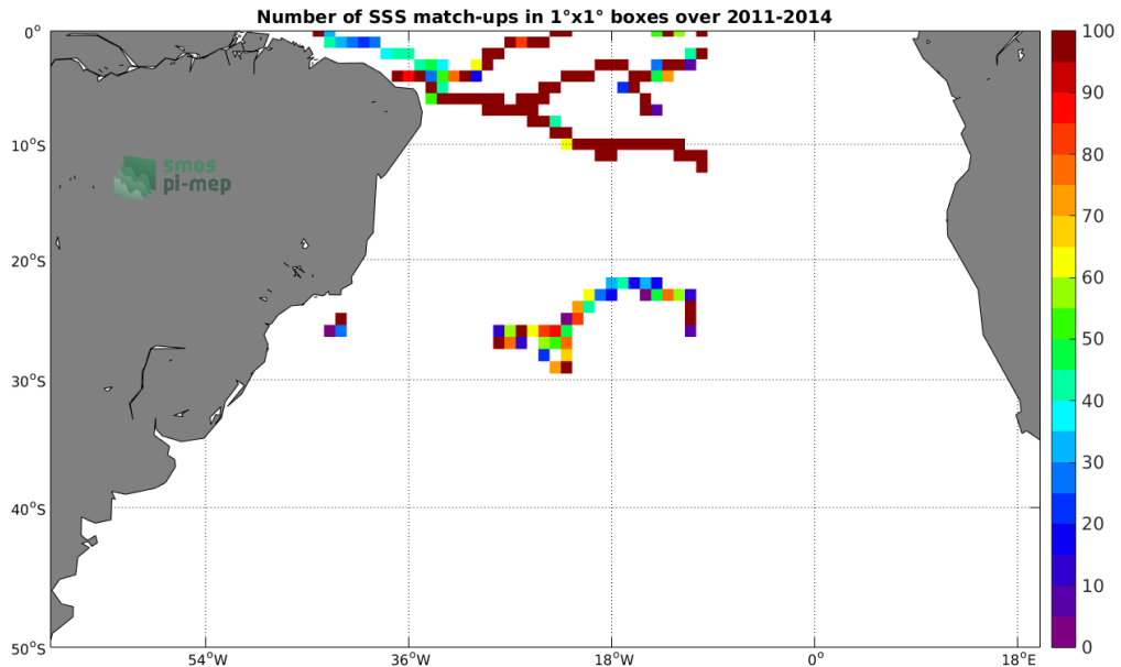
Figure 3: Number of SSS match-ups between Surface drifters SSS and the Aquarius-L4-IPRC-V5-WEEKLY SSS product for the South Atlantic Ocean Pi-MEP region over 1^{\circ} \times 1^{\circ} boxes and for the full satellite product period.
