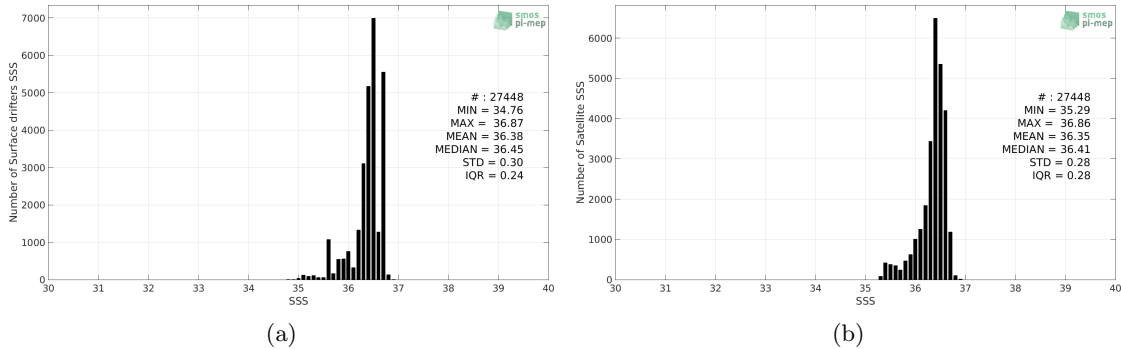
Figure 2: Histograms of SSS from Surface drifters (a) and Aquarius-L4-IPRC-V5-WEEKLY (b) considering all match-up pairs per bins of 0.1 over the South Atlantic Ocean Pi-MEP region and for the full satellite product period.
