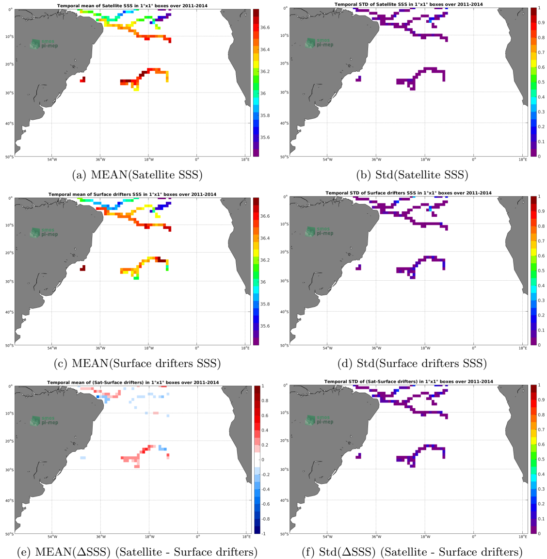
Figure 5: Temporal mean (left) and Std (right) of SSS from Aquarius-L4-IPRC-V5-WEEKLY (top), Surface drifters (middle), and of \Delta SSS (Satellite - Surface drifters). Only match-up pairs are used to generate these maps.
