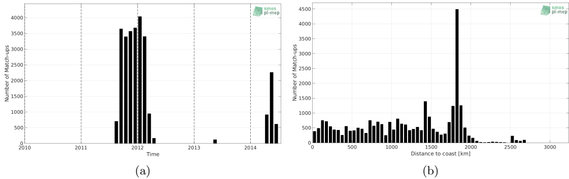
Figure 1: Number of match-ups between Surface drifters and Aquarius-L4-IPRC-V5-WEEKLY SSS as a function of time (a) and as function of the distance to coast (b) over the South Atlantic Ocean Pi-MEP region and for the full satellite product period.
