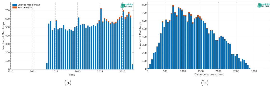
Figure 2: Number of match-ups between Argo and Aquarius SSS L4 OI v5 - Weekly (IPRC) SSS as a function of time (a) and as function of the distance to coast (b) over the South Atlantic Ocean Pi-MEP region and for the full satellite product period.
