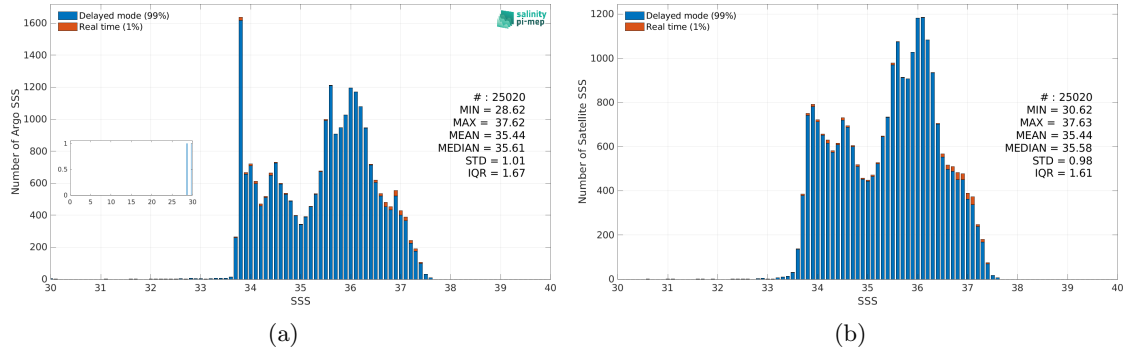
Figure 3: Histograms of SSS from Argo (a) and Aquarius SSS L4 OI v5 - Weekly (IPRC) (b) considering all match-up pairs per bins of 0.1 over the South Atlantic Ocean Pi-MEP region and for the full satellite product period.
