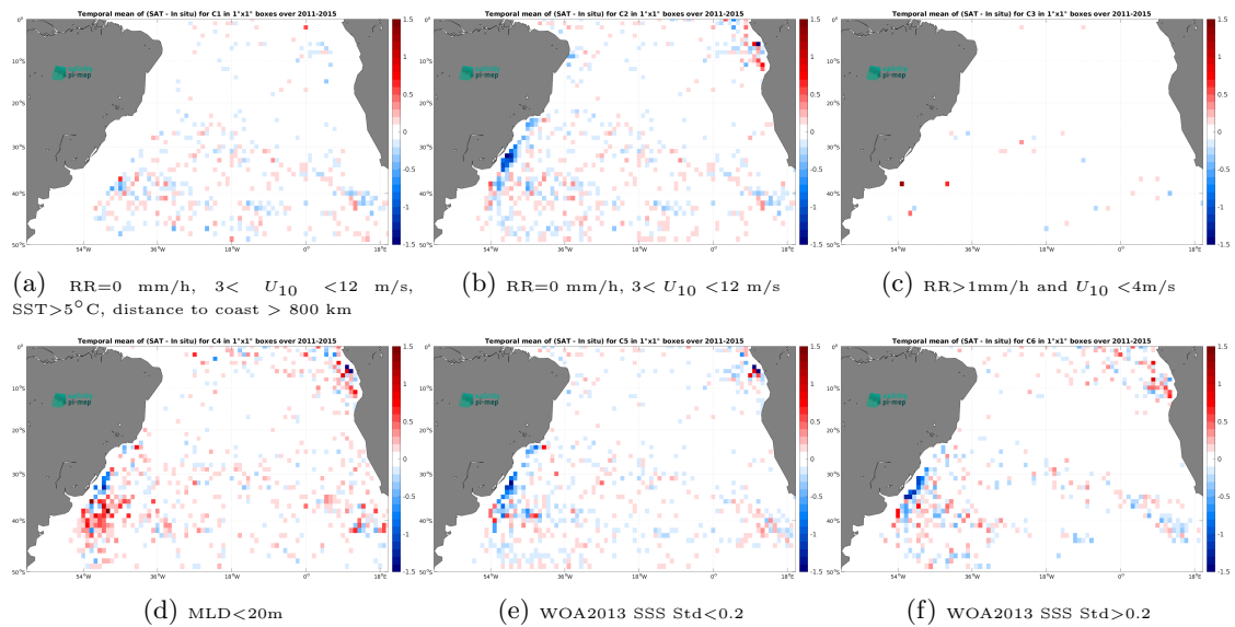
Figure 14: Temporal mean gridded over spatial boxes of size 1^\circ \times 1^\circ of \Delta SSS (Aquarius SSS L4 OI v5 - Weekly (IPRC) - Argo) for 6 different subdatasets corresponding to:RR=0 mm/h, 3 < U_{10} < 12 m/s, SST > 5^\circ\text{C} , distance to coast > 800 km (a), RR=0 mm/h, 3 < U_{10} < 12 m/s (b), RR > 1 mm/h and U_{10} < 4 m/s (c),MLD < 20 m (d),WOA2013 SSS Std < 0.2 (e),WOA2013 SSS Std > 0.2 (f).
