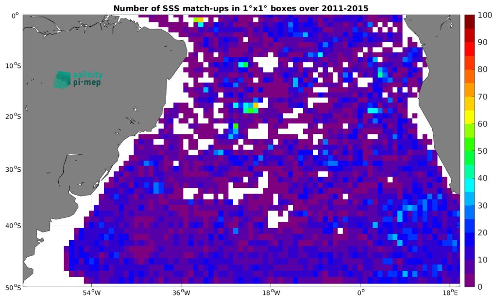
Figure 5: Number of SSS match-ups between Argo SSS and the Aquarius SSS L4 OI v5 - Weekly (IPRC) SSS product for the South Atlantic Ocean Pi-MEP region over 1^\circ \times 1^\circ boxes and for the full satellite product period.
