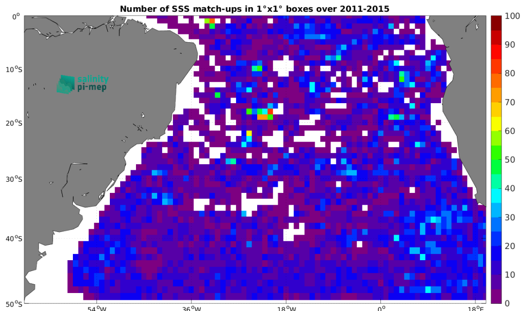
Figure 4: Number of SSS match-ups between Argo SSS and the Aquarius SSS L4 OI v5 - Weekly (IPRC) SSS product for the South Atlantic Ocean Pi-MEP region over 1^{\circ} \times 1^{\circ} boxes and for the full satellite product period.
