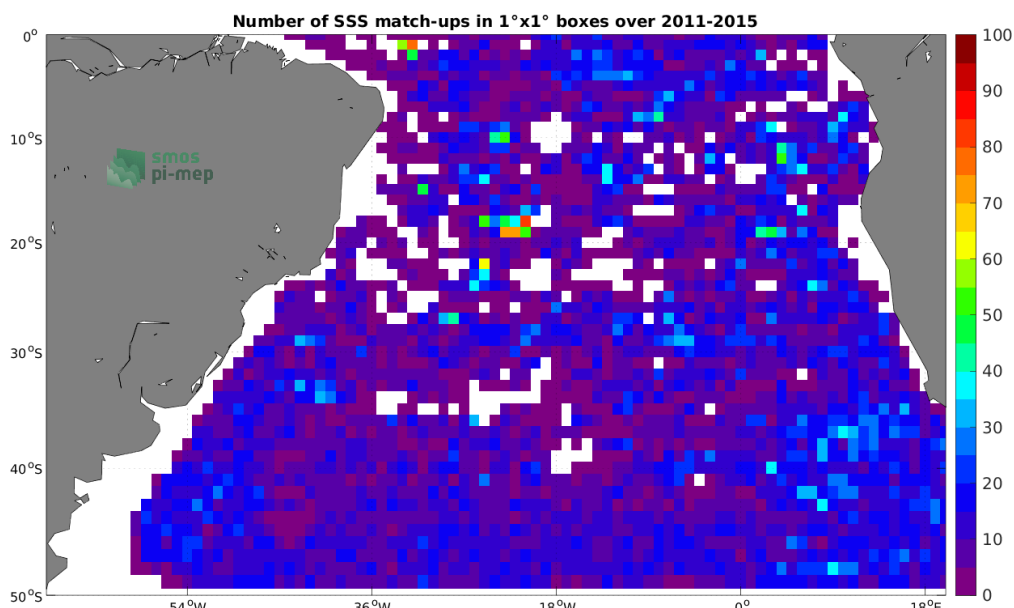
Figure 4: Number of SSS match-ups between Argo SSS and the Aquarius SSS L4 OI v5 - Weekly (IPRC) SSS product for the South Atlantic Ocean Pi-MEP region over 1^\circ \times 1^\circ boxes and for the full satellite product period.
