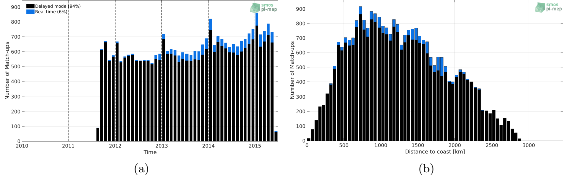
Figure 1: Number of match-ups between Argo and Aquarius SSS L4 OI v5 - Weekly (IPRC) SSS as a function of time (a) and as function of the distance to coast (b) over the South Atlantic Ocean Pi-MEP region and for the full satellite product period.
