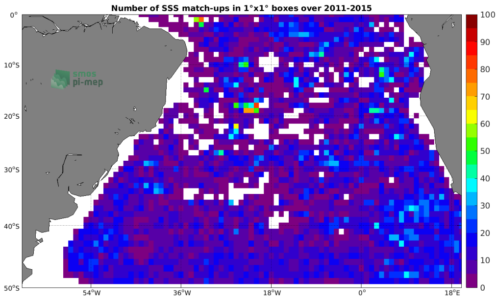
Figure 4: Number of SSS match-ups between Argo SSS and the Aquarius SSS L4 OI v5 - Weekly (IPRC) SSS product for the South Atlantic Ocean Pi-MEP region over 1°x1° boxes and for the full satellite product period.
