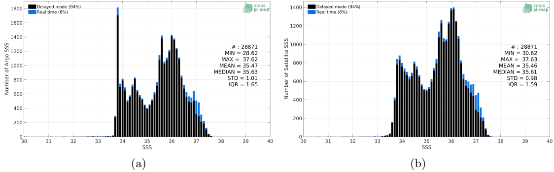
Figure 2: Histograms of SSS from Argo (a) and Aquarius SSS L4 OI v5 - Weekly (IPRC) (b) considering all match-up pairs per bins of 0.1 over the South Atlantic Ocean Pi-MEP region and for the full satellite product period.
