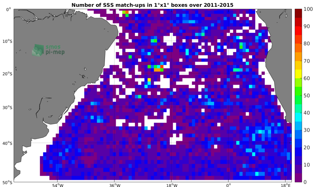
Figure 4: Number of SSS match-ups between Argo SSS and the Aquarius-L4-IPRC-V5-WEEKLY SSS product for the South Atlantic Ocean Pi-MEP region over 1°x1° boxes and for the full satellite product period.
