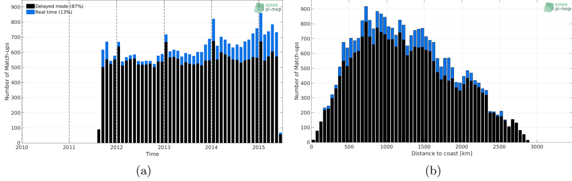
Figure 1: Number of match-ups between Argo and Aquarius-L4-IPRC-V5-WEEKLY SSS as a function of time (a) and as function of the distance to coast (b) over the South Atlantic Ocean Pi-MEP region and for the full satellite product period.
