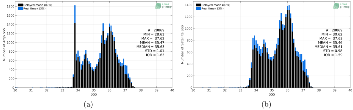
Figure 2: Histograms of SSS from Argo (a) and Aquarius-L4-IPRC-V5-WEEKLY (b) considering all match-up pairs per bins of 0.1 over the South Atlantic Ocean Pi-MEP region and for the full satellite product period.
