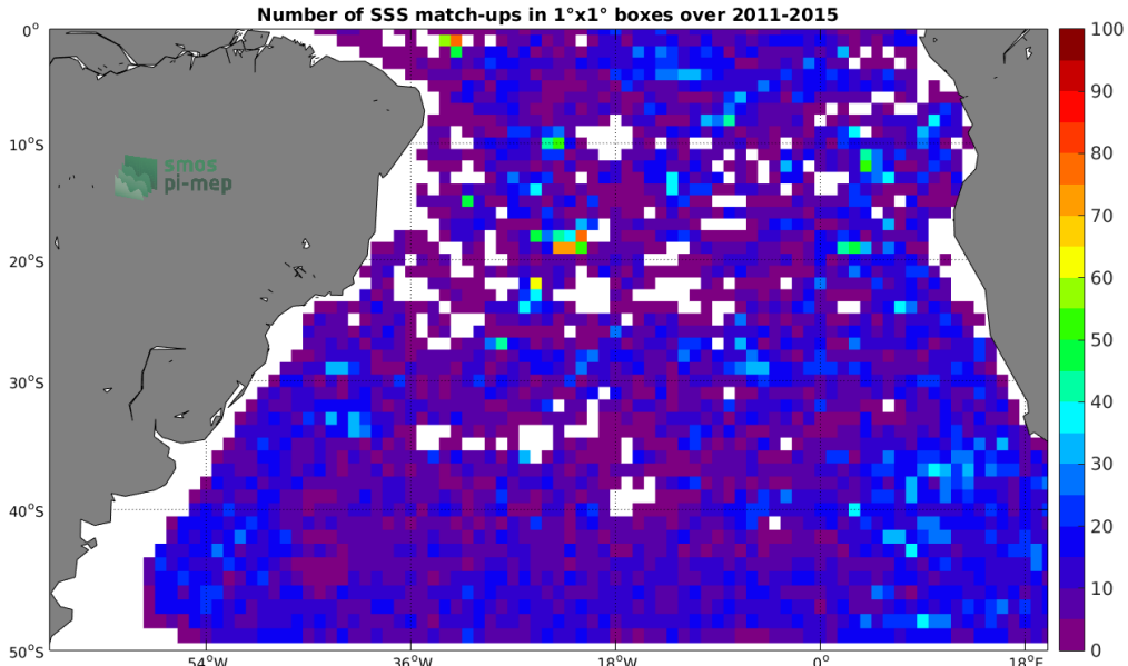
Figure 4: Number of SSS match-ups between Argo SSS and the Aquarius-L4-IPRC-V5-WEEKLY SSS product for the South Atlantic Ocean Pi-MEP region over 1^\circ \times 1^\circ boxes and for the full satellite product period.
