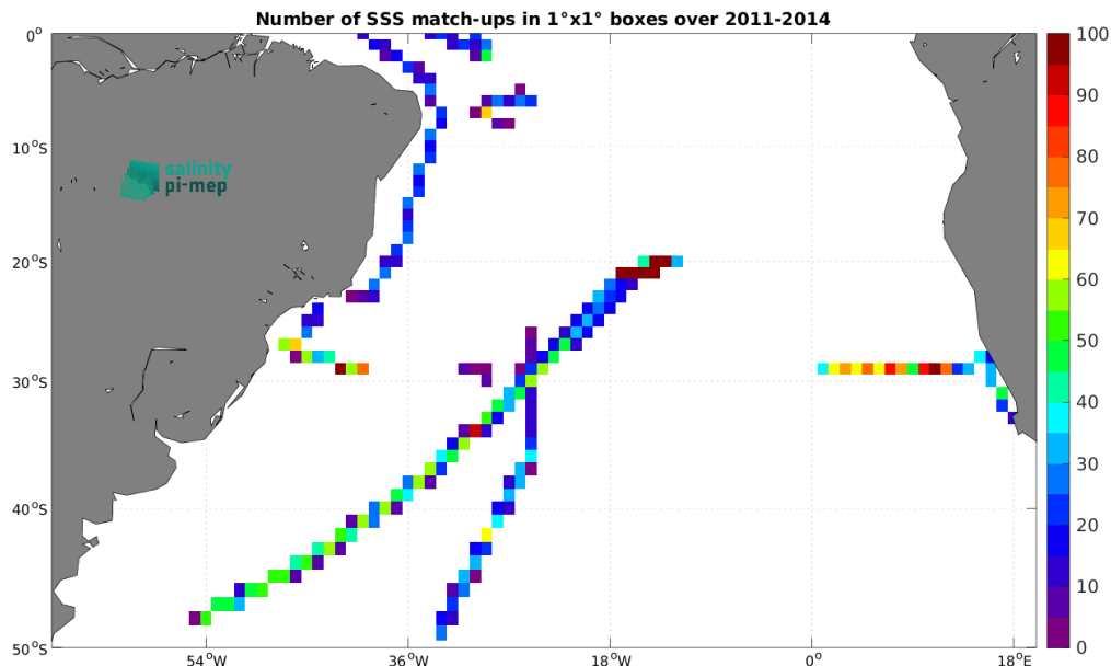
Figure 5: Number of SSS match-ups between TSG (SAMOS) SSS and the Aquarius SSS L4 OI v5 - Monthly (IPRC) SSS product for the South Atlantic Ocean Pi-MEP region over 1^\circ \times 1^\circ boxes and for the full satellite product period.
