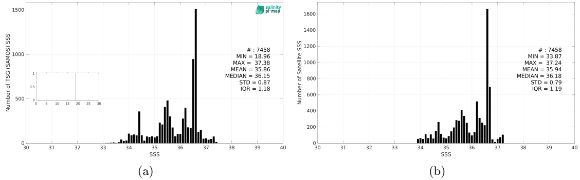
Figure 3: Histograms of SSS from TSG (SAMOS) (a) and Aquarius SSS L4 OI v5 - Monthly (IPRC) (b) considering all match-up pairs per bins of 0.1 over the South Atlantic Ocean Pi-MEP region and for the full satellite product period.
