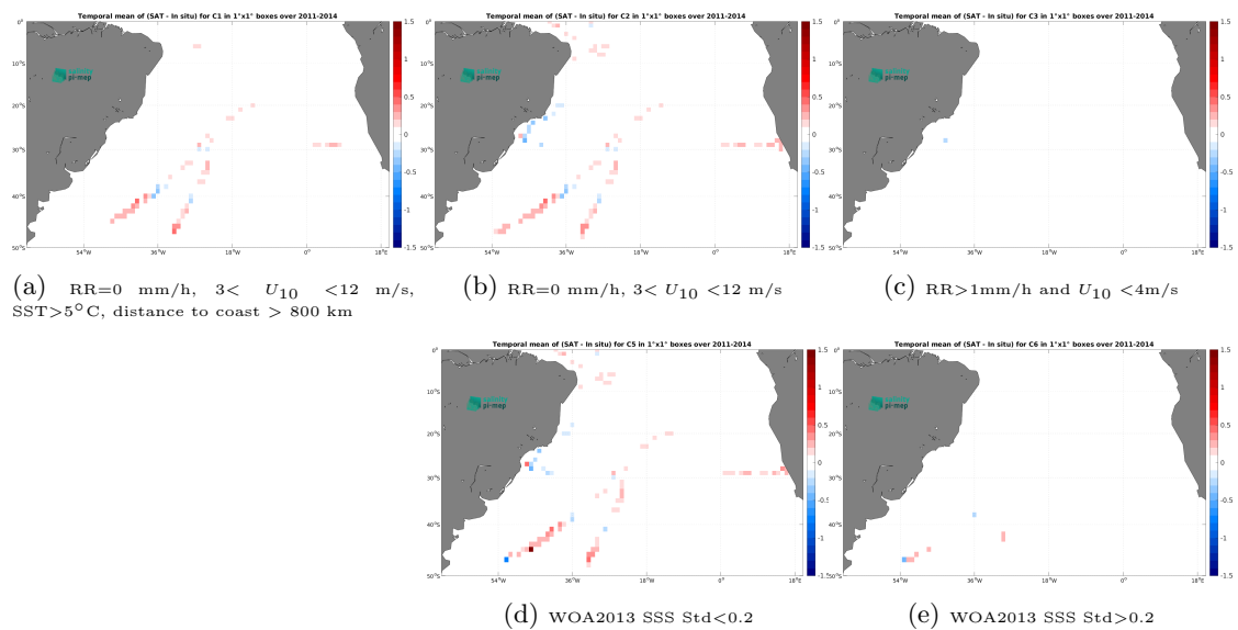
Figure 14: Temporal mean gridded over spatial boxes of size 1^\circ \times 1^\circ of \Delta SSS (Aquarius SSS L4 OI v5 - Monthly (IPRC) - TSG (SAMOS)) for 5 different subdatasets corresponding to:RR=0 mm/h, 3 < U_{10} < 12 m/s, SST >5^\circ\text{C} , distance to coast > 800 km (a), RR=0 mm/h, 3 < U_{10} < 12 m/s (b), RR >1 mm/h and U_{10} < 4 m/s (c), WOA2013 SSS Std <0.2 (d), WOA2013 SSS Std >0.2 (e).
