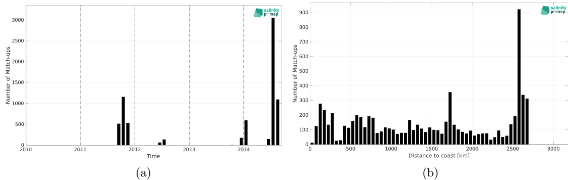
Figure 2: Number of match-ups between TSG (SAMOS) and Aquarius SSS L4 OI v5 - Monthly (IPRC) SSS as a function of time (a) and as function of the distance to coast (b) over the South Atlantic Ocean Pi-MEP region and for the full satellite product period.
