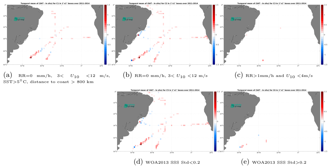
Figure 12: Temporal mean gridded over spatial boxes of size 1^\circ \times 1^\circ of \Delta\text{SSS} (Aquarius SSS L4 OI v5 - Monthly (IPRC) - TSG (SAMOS)) for 5 different subdatasets corresponding to:RR=0 mm/h, 3 < U_{10} < 12 m/s, SST >5^\circ\text{C} , distance to coast > 800 km (a), RR=0 mm/h, 3 < U_{10} < 12 m/s (b), RR >1 mm/h and U_{10} < 4 m/s (c), WOA2013 SSS Std <0.2 (d), WOA2013 SSS Std >0.2 (e).
