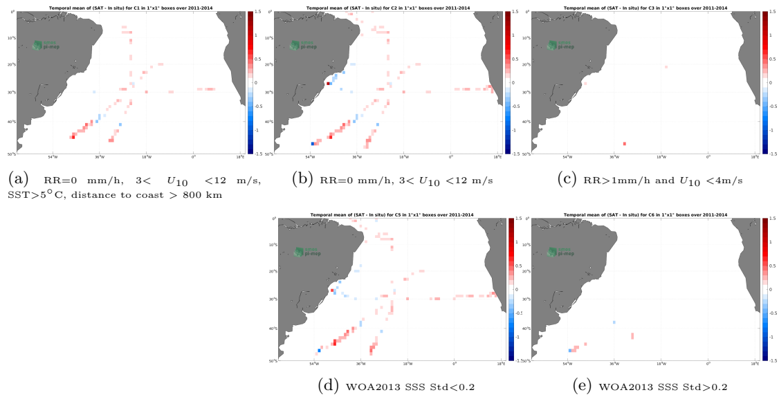
Figure 12: Temporal mean gridded over spatial boxes of size 1^\circ \times 1^\circ of \Delta\text{SSS} (Aquarius SSS L4 OI v5 - Monthly (IPRC) - TSG (SAMOS)) for 5 different subdatasets corresponding to: \text{RR}=0 mm/h, 3 < U_{10} < 12 m/s, \text{SST} > 5^\circ\text{C} , distance to coast > 800 km (a), \text{RR}=0 mm/h, 3 < U_{10} < 12 m/s (b), \text{RR} > 1 mm/h and U_{10} < 4 m/s (c), WOA2013 SSS Std < 0.2 (d), WOA2013 SSS Std > 0.2 (e).
