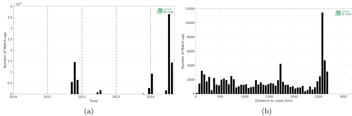
Figure 1: Number of match-ups between TSG (SAMOS) and Aquarius SSS L4 OI v5 - Monthly (IPRC) SSS as a function of time (a) and as function of the distance to coast (b) over the South Atlantic Ocean Pi-MEP region and for the full satellite product period.
