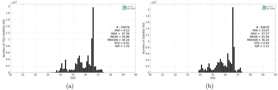
Figure 2: Histograms of SSS from TSG (SAMOS) (a) and Aquarius SSS L4 OI v5 - Monthly (IPRC) (b) considering all match-up pairs per bins of 0.1 over the South Atlantic Ocean Pi-MEP region and for the full satellite product period.
