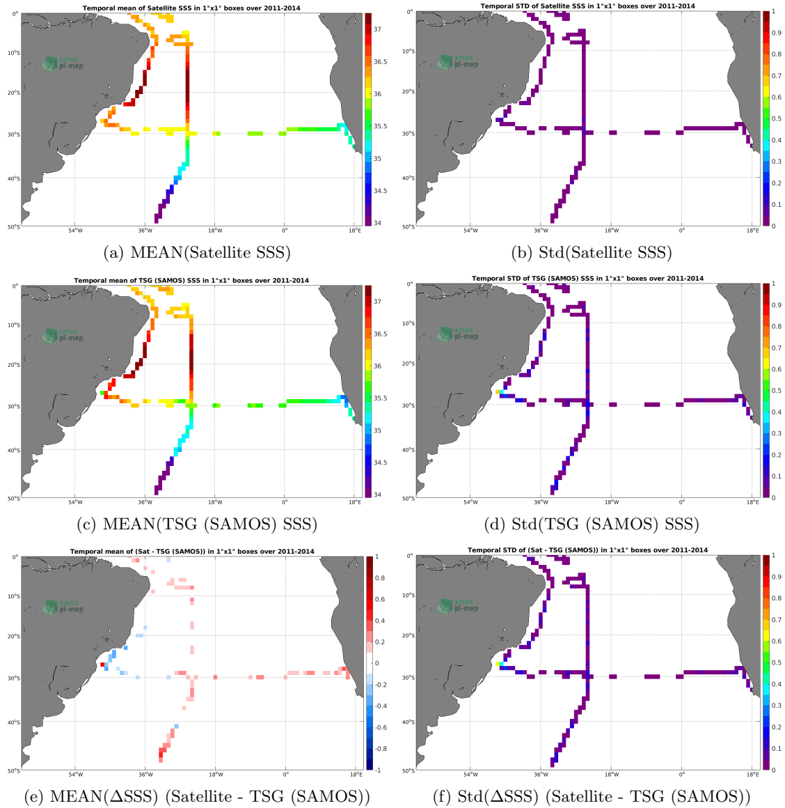
Figure 6: Temporal mean (left) and Std (right) of SSS from Aquarius SSS L4 OI v5 - Monthly (IPRC) (top), TSG (SAMOS) (middle), and of \Delta SSS (Satellite - TSG (SAMOS)). Only match-up pairs are used to generate these maps.
