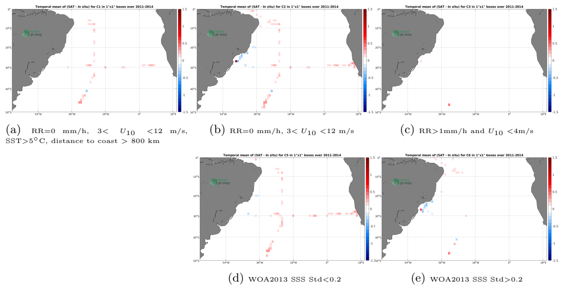
Figure 12: Temporal mean gridded over spatial boxes of size 1^\circ \times 1^\circ of \Delta SSS (Aquarius SSS L4 OI v5 - Monthly (IPRC) - TSG (SAMOS)) for 5 different subdatasets corresponding to:RR=0 mm/h, 3 < U_{10} < 12 m/s, SST > 5^\circ\text{C} , distance to coast > 800 km (a), RR=0 mm/h, 3 < U_{10} < 12 m/s (b), RR > 1 mm/h and U_{10} < 4 m/s (c), WOA2013 SSS Std < 0.2 (d), WOA2013 SSS Std > 0.2 (e).
