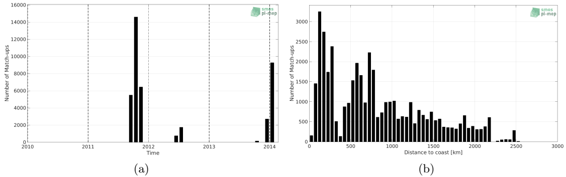
Figure 1: Number of match-ups between TSG (SAMOS) and Aquarius SSS L4 OI v5 - Monthly (IPRC) SSS as a function of time (a) and as function of the distance to coast (b) over the South Atlantic Ocean Pi-MEP region and for the full satellite product period.
