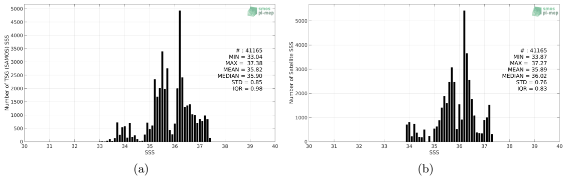
Figure 2: Histograms of SSS from TSG (SAMOS) (a) and Aquarius SSS L4 OI v5 - Monthly (IPRC) (b) considering all match-up pairs per bins of 0.1 over the South Atlantic Ocean Pi-MEP region and for the full satellite product period.
