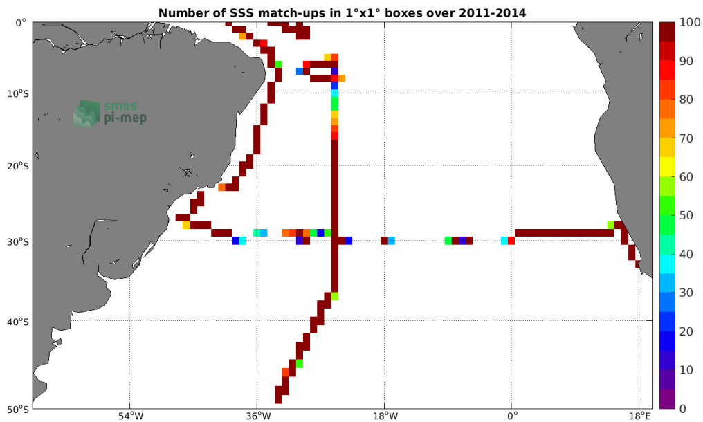
Figure 4: Number of SSS match-ups between TSG (SAMOS) SSS and the Aquarius SSS L4 OI v5 - Monthly (IPRC) SSS product for the South Atlantic Ocean Pi-MEP region over 1^\circ \times 1^\circ boxes and for the full satellite product period.
