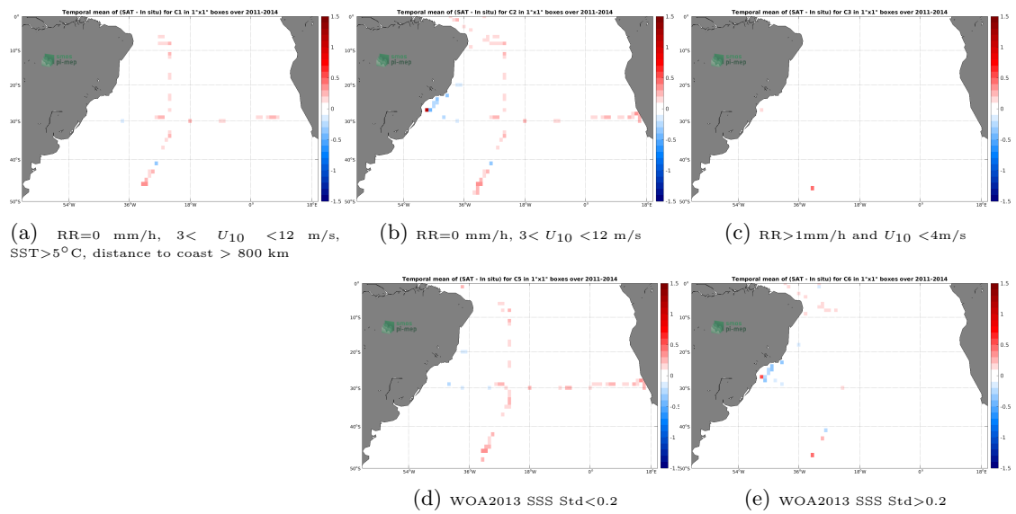
Figure 12: Temporal mean gridded over spatial boxes of size 1°x1° of \Delta SSS (Aquarius SSS L4 OI v5 - Monthly (IPRC) - TSG (SAMOS)) for 5 different subdatasets corresponding to: RR=0 mm/h, 3 < U_{10} < 12 m/s, SST > 5°C, distance to coast > 800 km (a), RR=0 mm/h, 3 < U_{10} < 12 m/s (b), RR > 1mm/h and U_{10} < 4 m/s (c), WOA2013 SSS Std < 0.2 (d), WOA2013 SSS Std > 0.2 (e).
