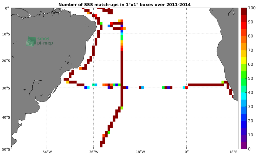
Figure 4: Number of SSS match-ups between TSG-SAMOS SSS and the Aquarius-L4-IPRC-V5-MONTHLY SSS product for the South Atlantic Ocean Pi-MEP region over 1°x1° boxes and for the full satellite product period.
