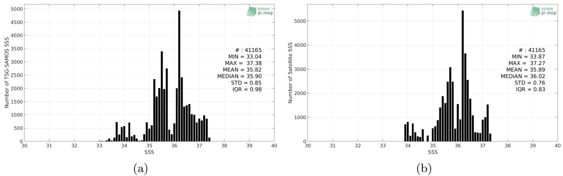
Figure 2: Histograms of SSS from TSG-SAMOS (a) and Aquarius-L4-IPRC-V5-MONTHLY (b) considering all match-up pairs per bins of 0.1 over the South Atlantic Ocean Pi-MEP region and for the full satellite product period.
