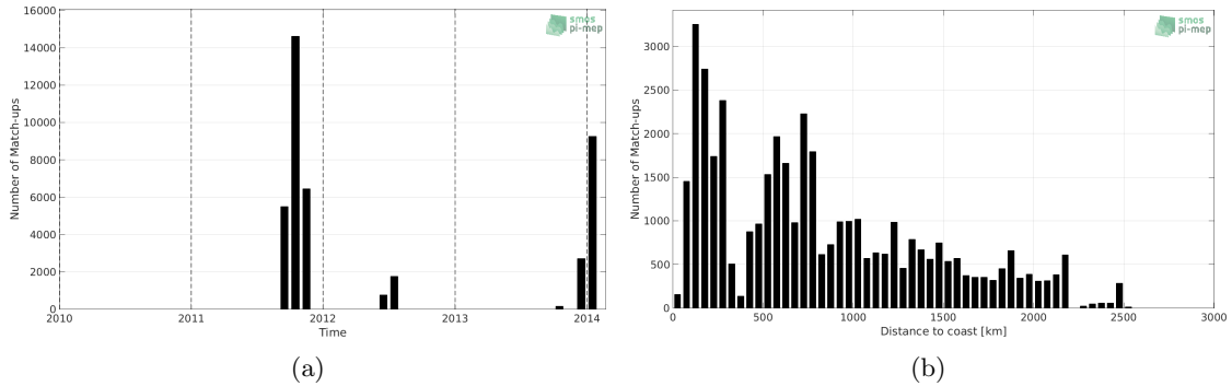
Figure 1: Number of match-ups between TSG-SAMOS and Aquarius-L4-IPRC-V5-MONTHLY SSS as a function of time (a) and as function of the distance to coast (b) over the South Atlantic Ocean Pi-MEP region and for the full satellite product period.
