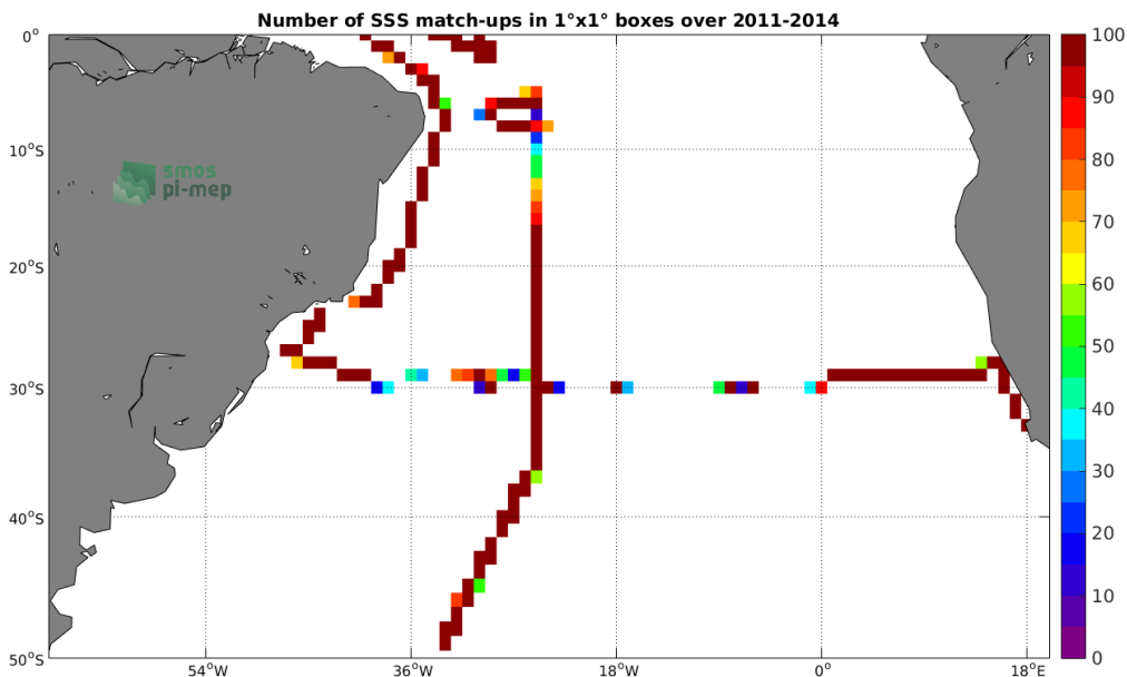
Figure 4: Number of SSS match-ups between TSG-SAMOS SSS and the Aquarius-L4-IPRC-V5-MONTHLY SSS product for the South Atlantic Ocean Pi-MEP region over 1^\circ \times 1^\circ boxes and for the full satellite product period.
