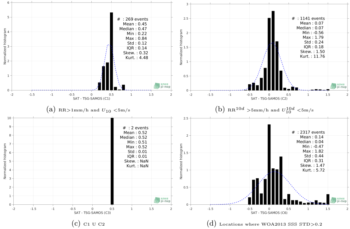
Figure 13: Normalized histogram of \Delta\text{SSS} (Aquarius-L4-IPRC-V5-MONTHLY - TSG-SAMOS) for 6 different subdatasets corresponding to: RR > 1mm/h and U_{10} < 5\text{m/s} (a), RR^{10d} > 5\text{mm/h} and U_{10}^{10d} < 5\text{m/s} (b), C1 U C2 (c), Locations where WOA2013 SSS STD > 0.2 (d).
