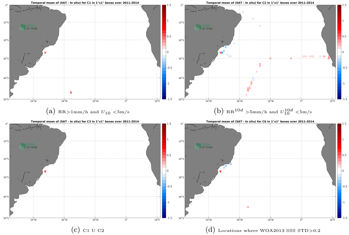
Figure 12: Temporal mean gridded over spatial boxes of size 1^\circ \times 1^\circ of \Delta SSS (Aquarius-L4-IPRC-V5-MONTHLY - TSG-SAMOS) for 4 different subdatasets corresponding to: RR > 1mm/h and U_{10} < 5\text{m/s} (a), RR^{10d} > 5\text{mm/h} and U_{10}^{10d} < 5\text{m/s} (b), C1 U C2 (c), Locations where WOA2013 SSS STD > 0.2 (d).
