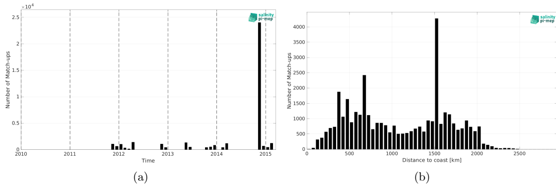
Figure 2: Number of match-ups between TSG (Polarstern) and Aquarius SSS L4 OI v5 - Monthly (IPRC) SSS as a function of time (a) and as function of the distance to coast (b) over the South Atlantic Ocean Pi-MEP region and for the full satellite product period.
