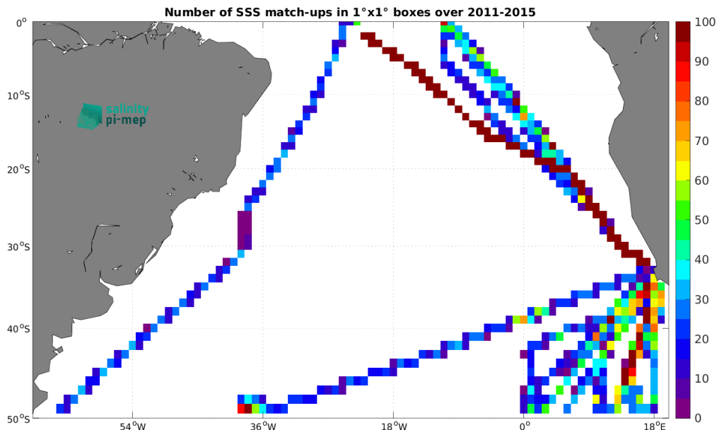
Figure 5: Number of SSS match-ups between TSG (Polarstern) SSS and the Aquarius SSS L4 OI v5 - Monthly (IPRC) SSS product for the South Atlantic Ocean Pi-MEP region over 1^\circ \times 1^\circ boxes and for the full satellite product period.
