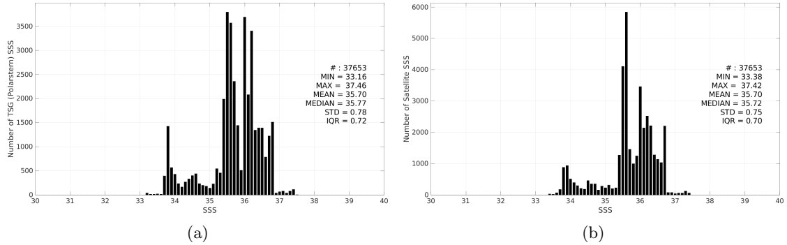
Figure 3: Histograms of SSS from TSG (Polarstern) (a) and Aquarius SSS L4 OI v5 - Monthly (IPRC) (b) considering all match-up pairs per bins of 0.1 over the South Atlantic Ocean Pi-MEP region and for the full satellite product period.
