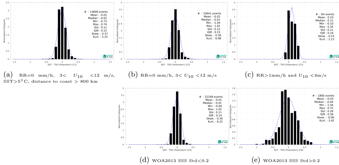
Figure 15: Normalized histogram of \Delta\text{SSS} (Aquarius SSS L4 OI v5 - Monthly (IPRC) - TSG (Polarstern)) for 5 different subdatasets corresponding to: RR=0 mm/h, 3 < U_{10} < 12 m/s, SST>5°C, distance to coast > 800 km (a), RR=0 mm/h, 3 < U_{10} < 12 m/s (b), RR>1mm/h and U_{10} < 4 m/s (c), WOA2013 SSS Std<0.2 (d), WOA2013 SSS Std>0.2 (e).
