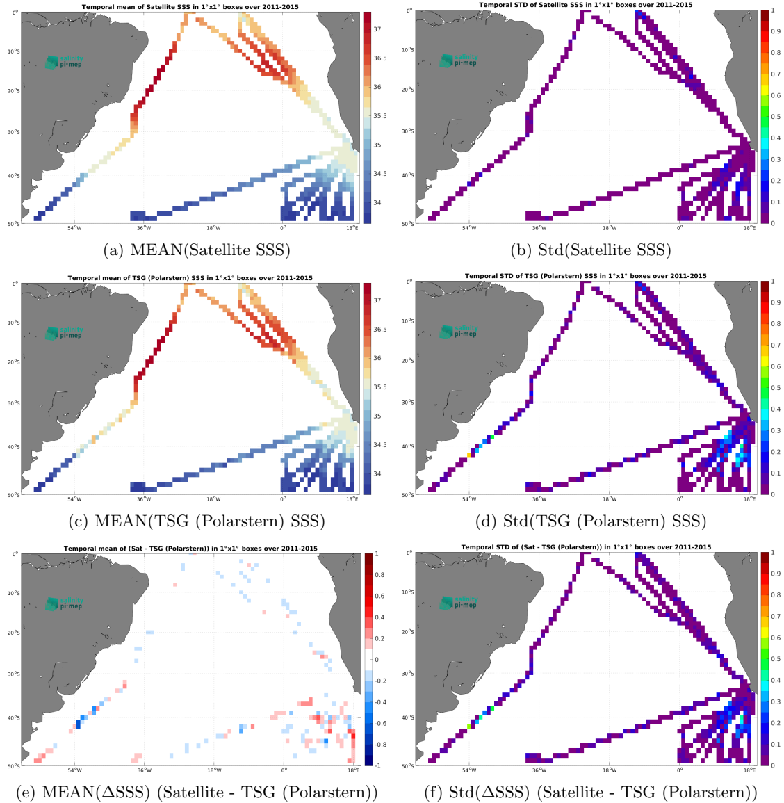
Figure 7: Temporal mean (left) and Std (right) of SSS from Aquarius SSS L4 OI v5 - Monthly (IPRC) (top), TSG (Polarstern) (middle), and of \Delta SSS (Satellite - TSG (Polarstern)). Only match-up pairs are used to generate these maps.
