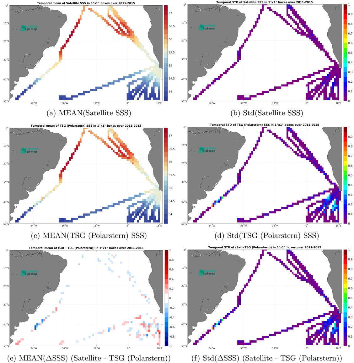
Figure 6: Temporal mean (left) and Std (right) of SSS from Aquarius SSS L4 OI v5 - Monthly (IPRC) (top), TSG (Polarstern) (middle), and of \Delta SSS (Satellite - TSG (Polarstern)). Only match-up pairs are used to generate these maps.
