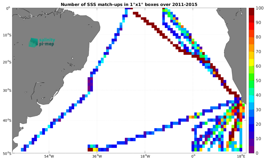
Figure 4: Number of SSS match-ups between TSG (Polarstern) SSS and the Aquarius SSS L4 OI v5 - Monthly (IPRC) SSS product for the South Atlantic Ocean Pi-MEP region over 1^\circ \times 1^\circ boxes and for the full satellite product period.
