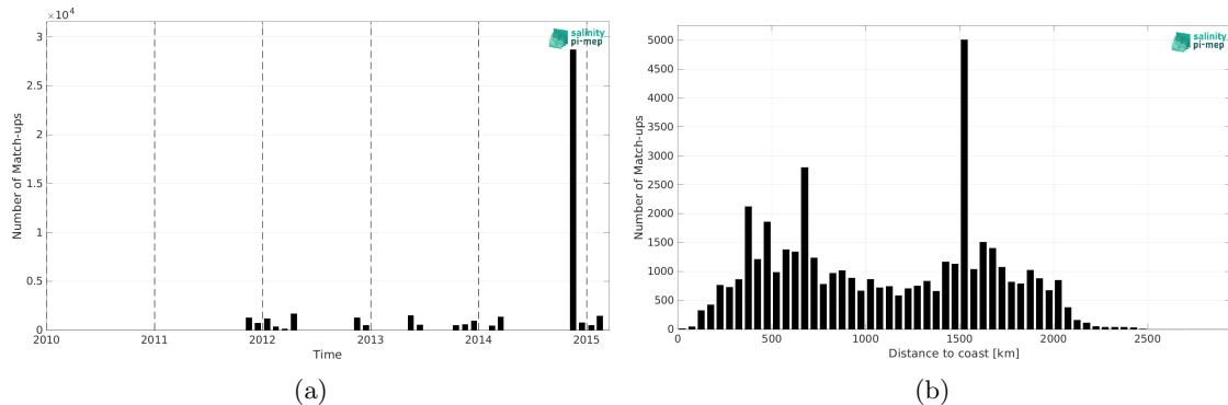
Figure 1: Number of match-ups between TSG (Polarstern) and Aquarius SSS L4 OI v5 - Monthly (IPRC) SSS as a function of time (a) and as function of the distance to coast (b) over the South Atlantic Ocean Pi-MEP region and for the full satellite product period.
