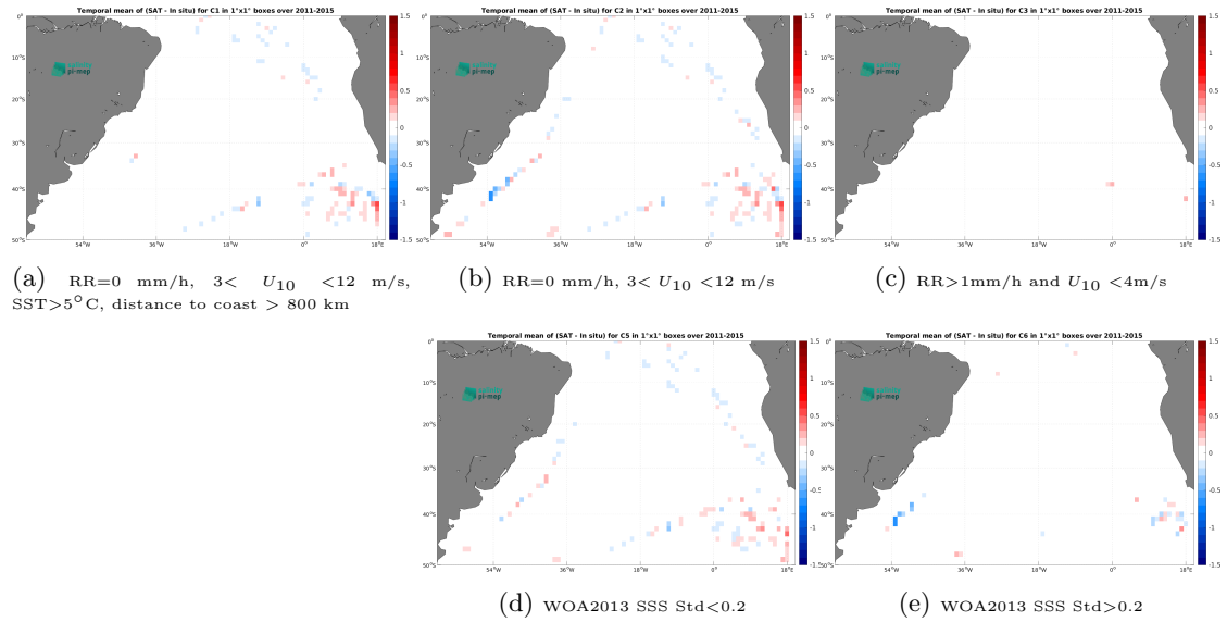
Figure 12: Temporal mean gridded over spatial boxes of size 1^\circ \times 1^\circ of \Delta SSS (Aquarius SSS L4 OI v5 - Monthly (IPRC) - TSG (Polarstern)) for 5 different subdatasets corresponding to:RR=0 mm/h, 3 < U_{10} < 12 m/s, SST >5^\circ\text{C} , distance to coast > 800 km (a), RR=0 mm/h, 3 < U_{10} < 12 m/s (b), RR >1 mm/h and U_{10} < 4 m/s (c), WOA2013 SSS Std <0.2 (d), WOA2013 SSS Std >0.2 (e).
