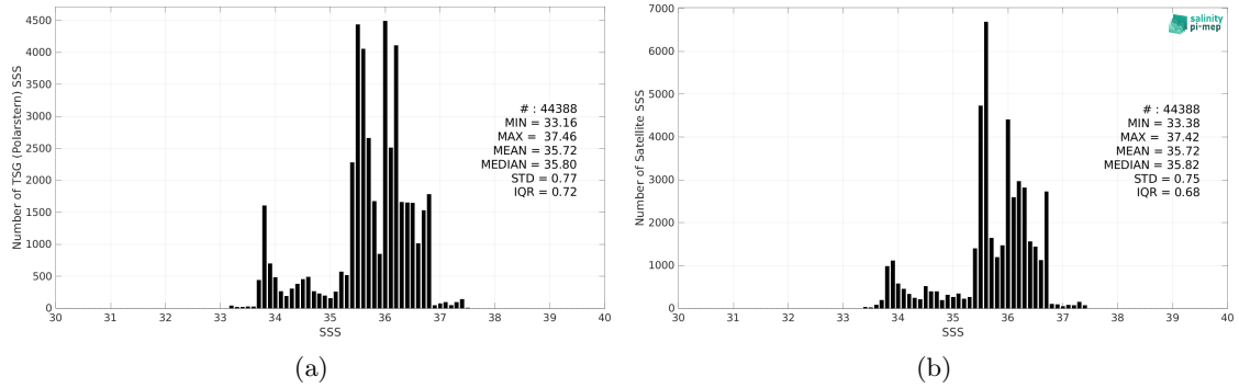
Figure 2: Histograms of SSS from TSG (Polarstern) (a) and Aquarius SSS L4 OI v5 - Monthly (IPRC) (b) considering all match-up pairs per bins of 0.1 over the South Atlantic Ocean Pi-MEP region and for the full satellite product period.
