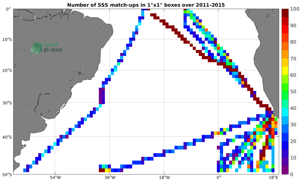
Figure 4: Number of SSS match-ups between TSG (Polarstern) SSS and the Aquarius SSS L4 OI v5 - Monthly (IPRC) SSS product for the South Atlantic Ocean Pi-MEP region over 1°x1° boxes and for the full satellite product period.
