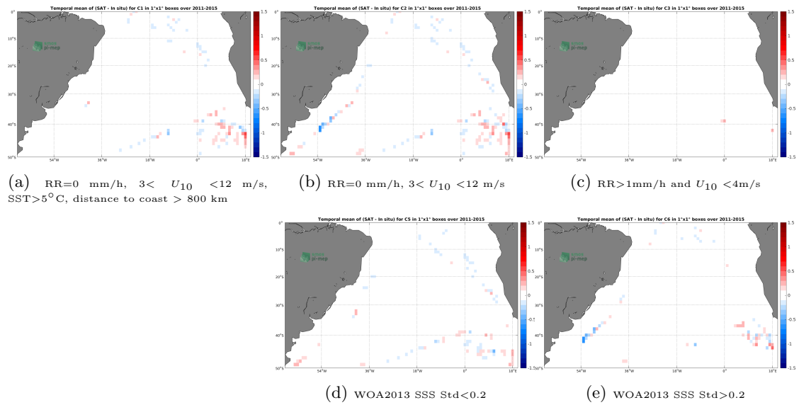
Figure 12: Temporal mean gridded over spatial boxes of size 1^\circ \times 1^\circ of \Delta SSS (Aquarius-L4-IPRC-V5-MONTHLY - TSG-POLARSTERN) for 5 different subdatasets corresponding to:RR=0 mm/h, 3 < U_{10} < 12 m/s, SST >5^\circ C, distance to coast > 800 km (a), RR=0 mm/h, 3 < U_{10} < 12 m/s (b), RR >1 mm/h and U_{10} < 4 m/s (c), WOA2013 SSS Std <0.2 (d), WOA2013 SSS Std >0.2 (e).
