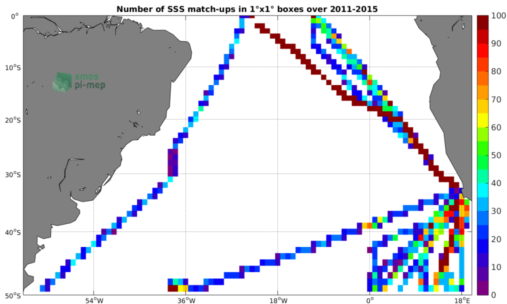
Figure 4: Number of SSS match-ups between TSG-POLARSTERN SSS and the Aquarius-L4-IPRC-V5-MONTHLY SSS product for the South Atlantic Ocean Pi-MEP region over 1^\circ \times 1^\circ boxes and for the full satellite product period.
