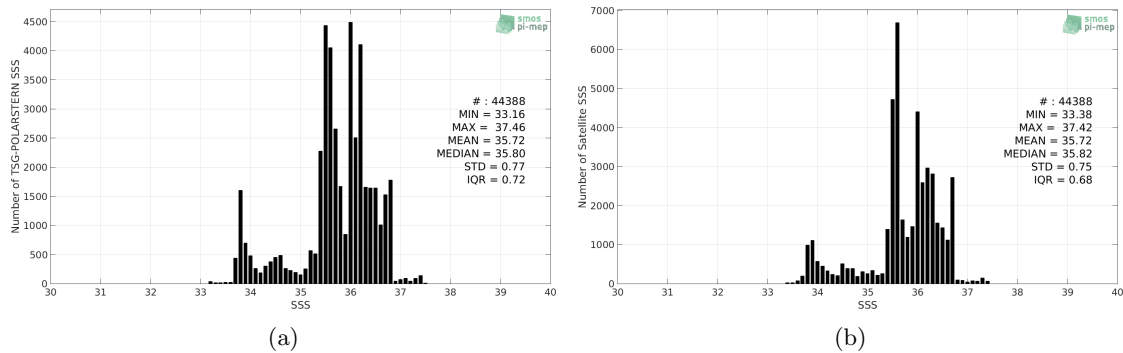
Figure 2: Histograms of SSS from TSG-POLARSTERN (a) and Aquarius-L4-IPRC-V5-MONTHLY (b) considering all match-up pairs per bins of 0.1 over the South Atlantic Ocean Pi-MEP region and for the full satellite product period.
