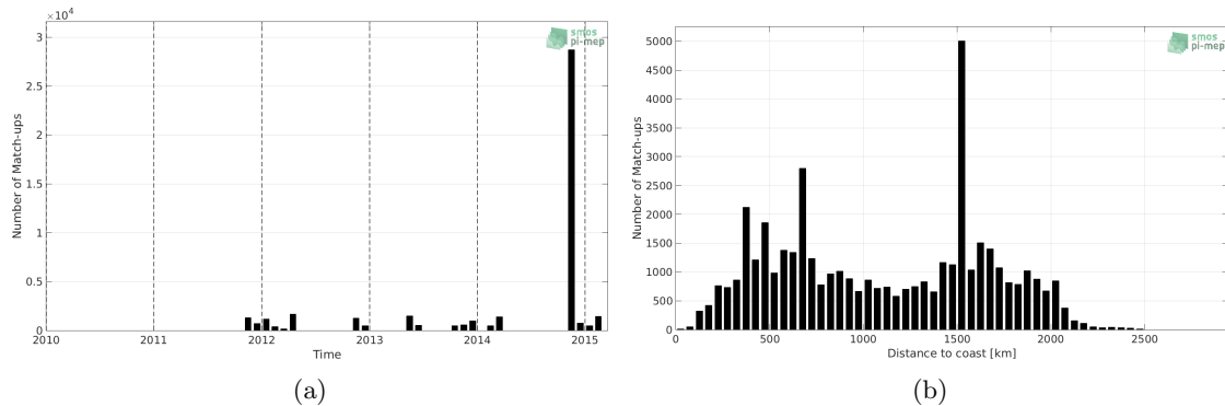
Figure 1: Number of match-ups between TSG-POLARSTERN and Aquarius-L4-IPRC-V5-MONTHLY SSS as a function of time (a) and as function of the distance to coast (b) over the South Atlantic Ocean Pi-MEP region and for the full satellite product period.
