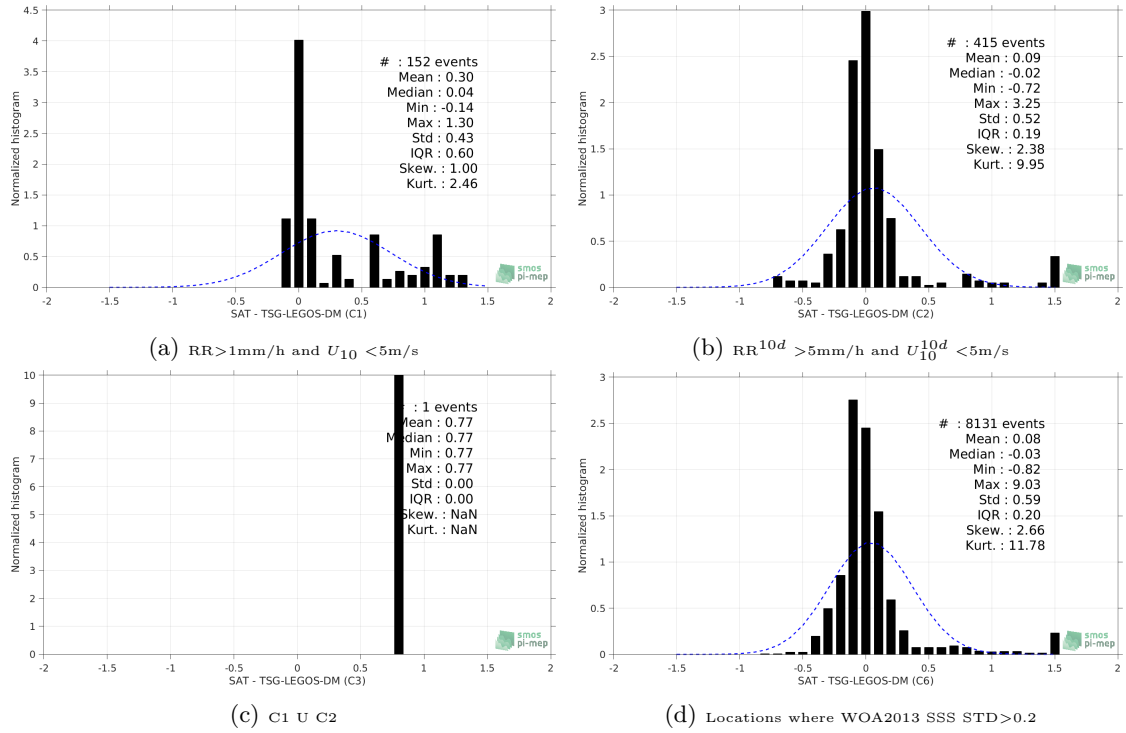
Figure 13: Normalized histogram of \Delta SSS (Aquarius-L4-IPRC-V5-MONTHLY - TSG-LEGOS-DM) for 6 different subdatasets corresponding to: RR > 1mm/h and U_{10} < 5 m/s (a), RR^{10d} > 5 mm/h and U_{10}^{10d} < 5 m/s (b), C1 U C2 (c), Locations where WOA2013 SSS STD > 0.2 (d).
