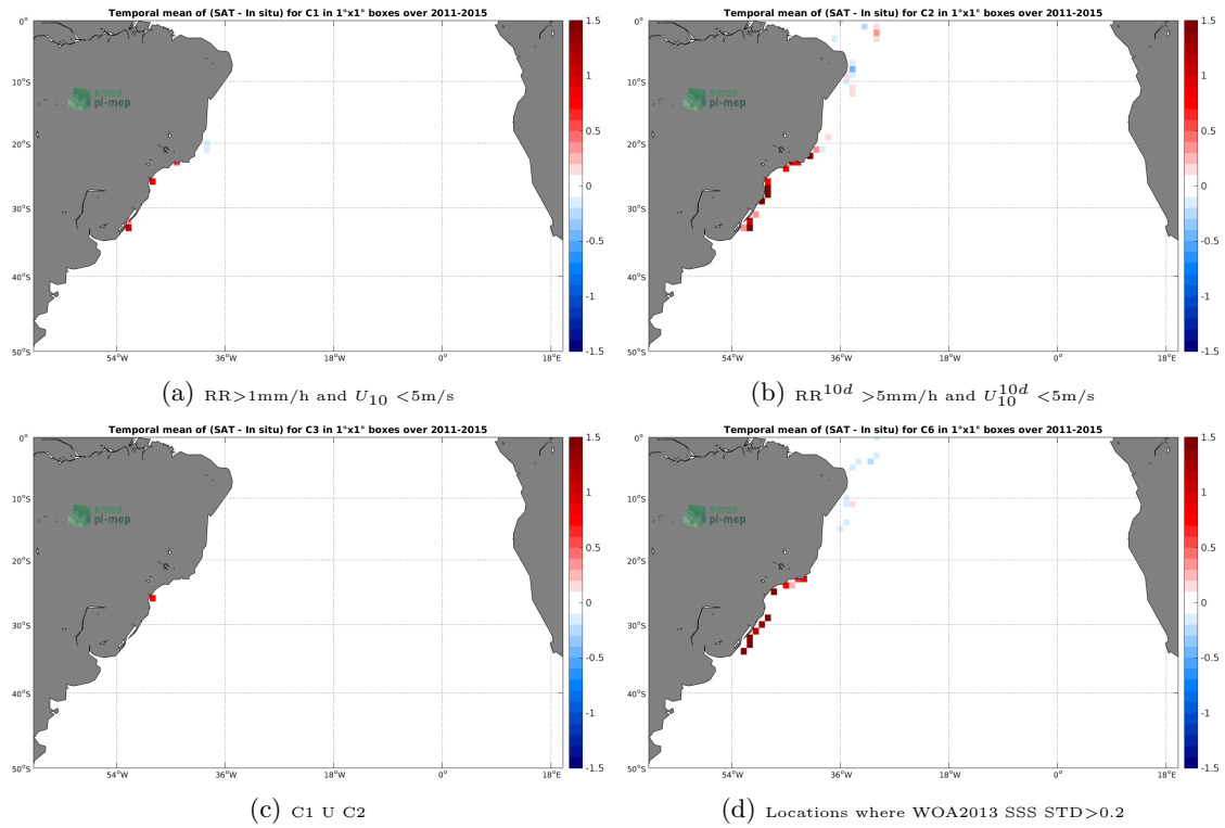
Figure 12: Temporal mean gridded over spatial boxes of size 1^\circ \times 1^\circ of \Delta SSS (Aquarius-L4-IPRC-V5-MONTHLY - TSG-LEGOS-DM) for 4 different subdatasets corresponding to: RR > 1mm/h and U_{10} < 5\text{m/s} (a), RR^{10d} > 5\text{mm/h} and U_{10}^{10d} < 5\text{m/s} (b), C1 U C2 (c), Locations where WOA2013 SSS STD > 0.2 (d).
