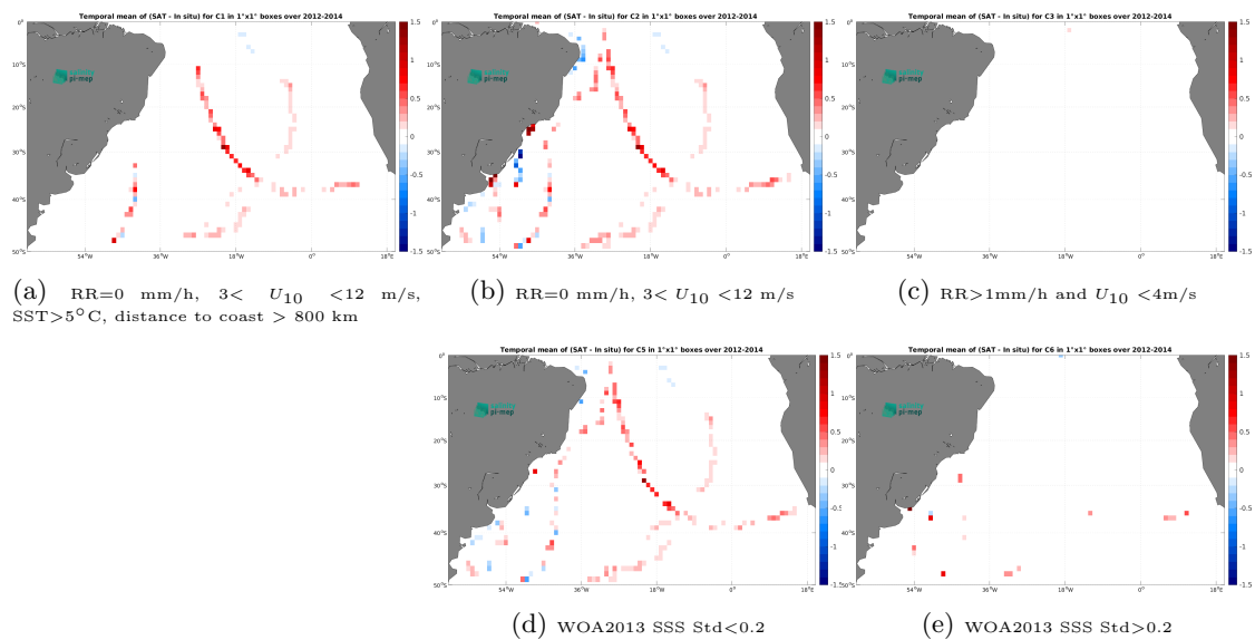
Figure 14: Temporal mean gridded over spatial boxes of size 1^\circ \times 1^\circ of \Delta\text{SSS} (Aquarius SSS L4 OI v5 - Monthly (IPRC) - TSG (GOSUD-Sailing-ship)) for 5 different subdatasets corresponding to:RR=0 mm/h, 3 < U_{10} < 12 m/s, SST >5^\circ\text{C} , distance to coast > 800 km (a), RR=0 mm/h, 3 < U_{10} < 12 m/s (b), RR >1 mm/h and U_{10} < 4 m/s (c), WOA2013 SSS Std <0.2 (d), WOA2013 SSS Std >0.2 (e).
