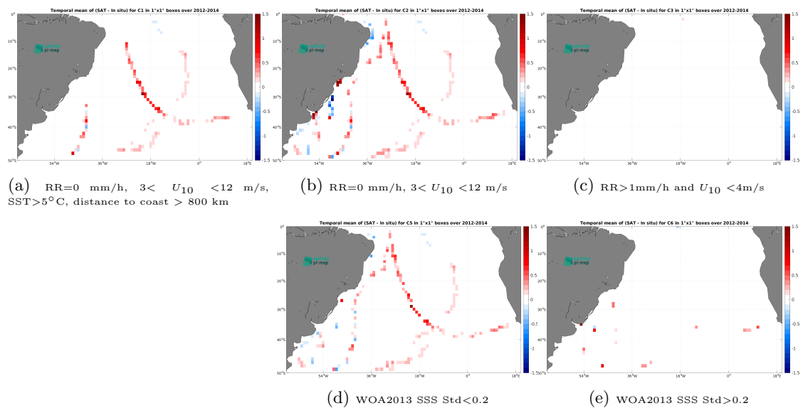
Figure 14: Temporal mean gridded over spatial boxes of size 1^\circ \times 1^\circ of \Delta\text{SSS} (Aquarius SSS L4 OI v5 - Monthly (IPRC) - TSG (GOSUD-Sailing-ship)) for 5 different subdatasets corresponding to:RR=0 mm/h, 3 < U_{10} < 12 m/s, SST >5^\circ\text{C} , distance to coast > 800 km (a), RR=0 mm/h, 3 < U_{10} < 12 m/s (b), RR >1 mm/h and U_{10} < 4 m/s (c), WOA2013 SSS Std <0.2 (d), WOA2013 SSS Std >0.2 (e).
