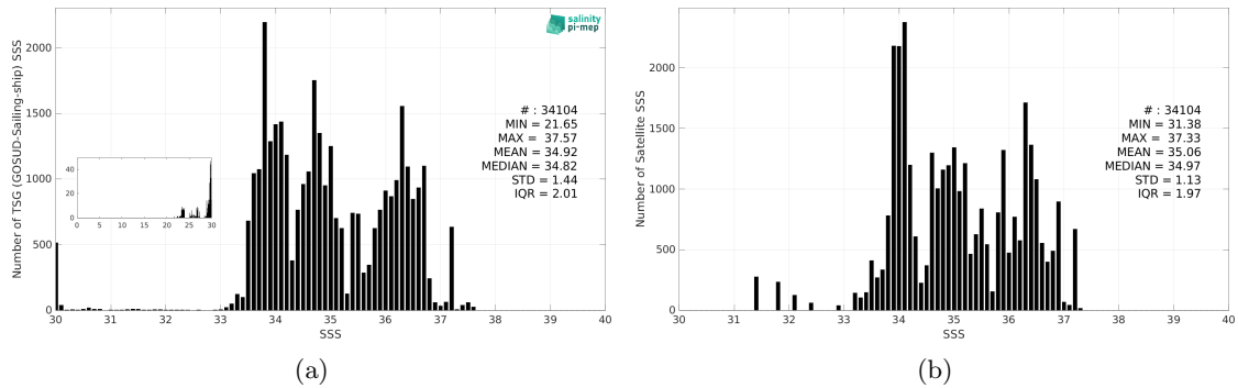
Figure 3: Histograms of SSS from TSG (GOSUD-Sailing-ship) (a) and Aquarius SSS L4 OI v5 - Monthly (IPRC) (b) considering all match-up pairs per bins of 0.1 over the South Atlantic Ocean Pi-MEP region and for the full satellite product period.
