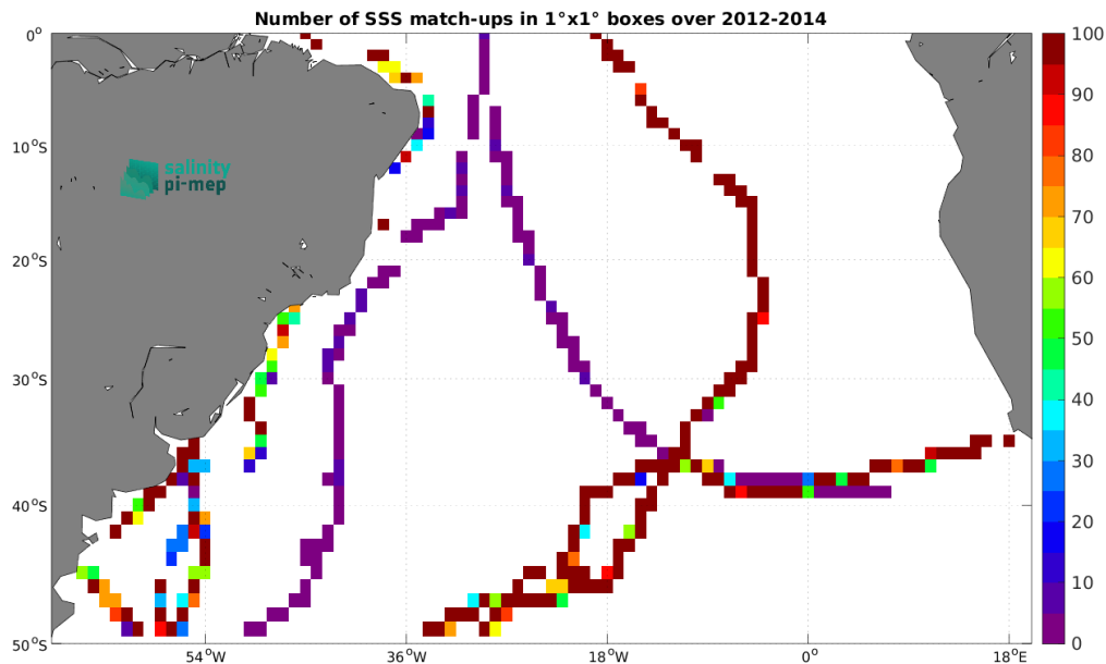
Figure 5: Number of SSS match-ups between TSG (GOSUD-Sailing-ship) SSS and the Aquarius SSS L4 OI v5 - Monthly (IPRC) SSS product for the South Atlantic Ocean Pi-MEP region over 1^\circ \times 1^\circ boxes and for the full satellite product period.
