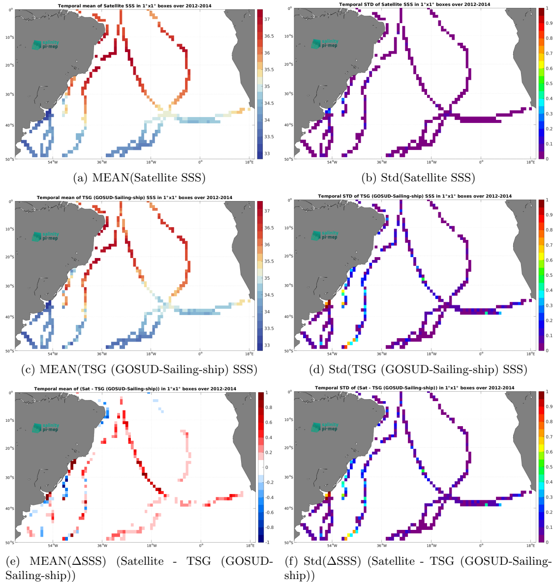
Figure 7: Temporal mean (left) and Std (right) of SSS from Aquarius SSS L4 OI v5 - Monthly (IPRC) (top), TSG (GOSUD-Sailing-ship) (middle), and of \Delta SSS (Satellite - TSG (GOSUD-Sailing-ship)). Only match-up pairs are used to generate these maps.
