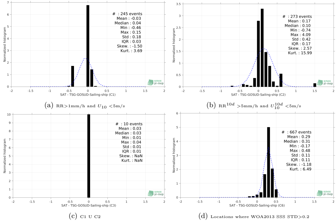
Figure 13: Normalized histogram of \Delta SSS (Aquarius-L4-IPRC-V5-MONTHLY - TSG-GOSUD-Sailing-ship) for 6 different subdatasets corresponding to: RR > 1\text{mm/h} and U_{10} < 5\text{m/s} (a), RR^{10d} > 5\text{mm/h} and U_{10}^{10d} < 5\text{m/s} (b), C1 U C2 (c), Locations where WOA2013 SSS STD > 0.2 (d).
