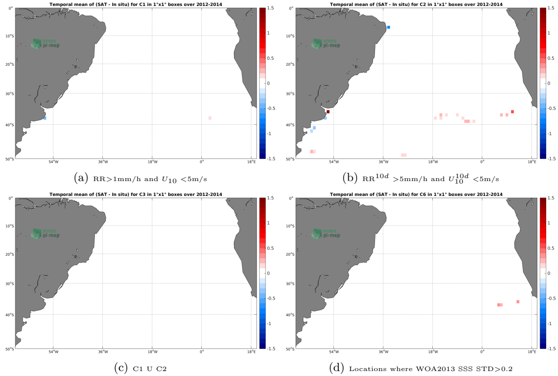
Figure 12: Temporal mean gridded over spatial boxes of size 1^\circ \times 1^\circ of \Delta SSS (Aquarius-L4-IPRC-V5-MONTHLY - TSG-GOSUD-Sailing-ship) for 4 different subdatasets corresponding to: RR > 1\text{mm/h} and U_{10} < 5\text{m/s} (a), RR^{10d} > 5\text{mm/h} and U_{10}^{10d} < 5\text{m/s} (b), C1 U C2 (c), Locations where WOA2013 SSS STD > 0.2 (d).
