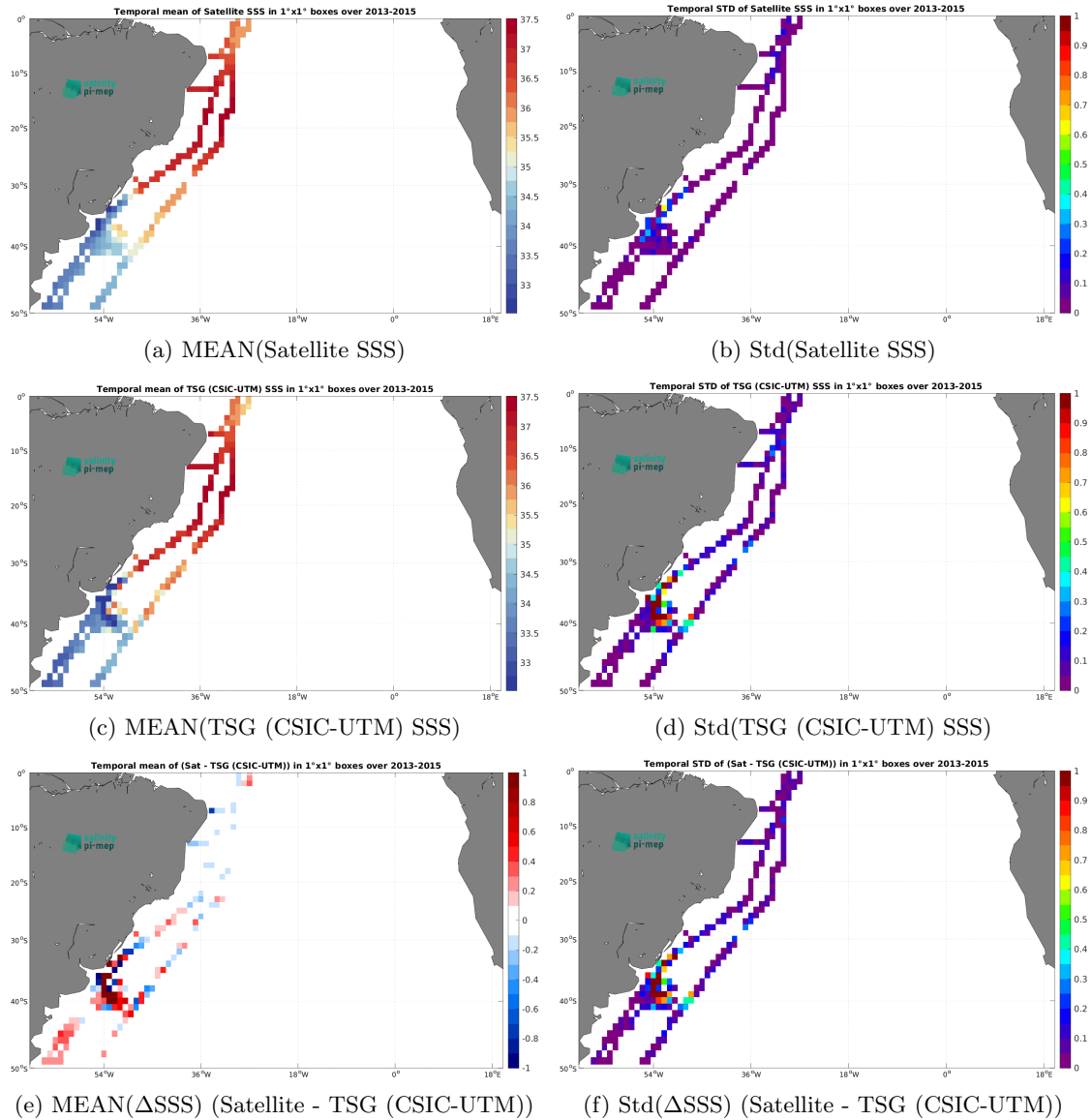
Figure 6: Temporal mean (left) and Std (right) of SSS from Aquarius SSS L4 OI v5 - Monthly (IPRC) (top), TSG (CSIC-UTM) (middle), and of \Delta SSS (Satellite - TSG (CSIC-UTM)). Only match-up pairs are used to generate these maps.
