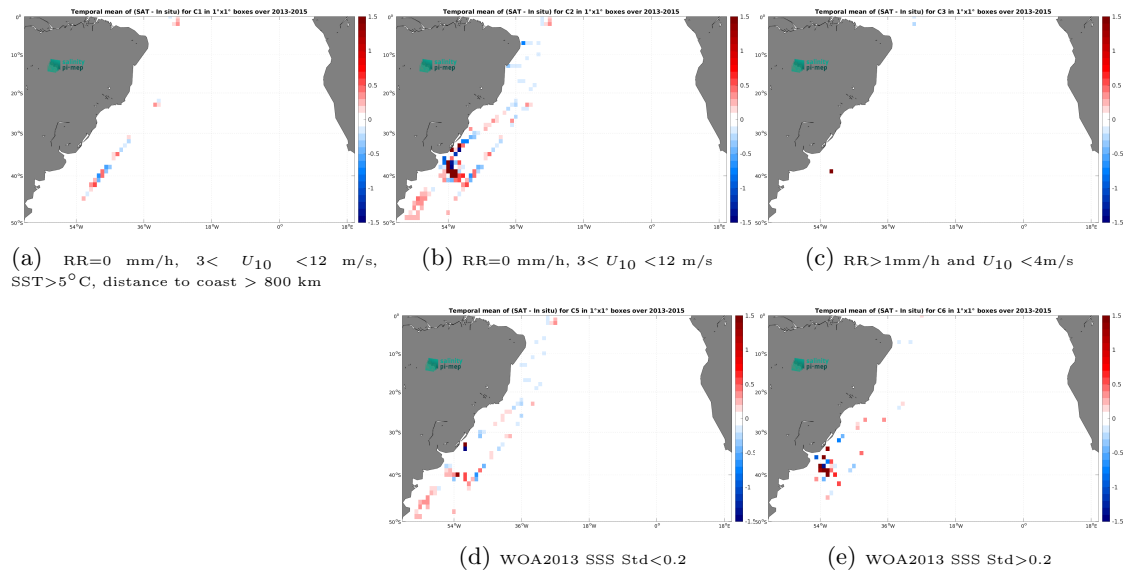
Figure 12: Temporal mean gridded over spatial boxes of size 1^\circ \times 1^\circ of \Delta\text{SSS} (Aquarius SSS L4 OI v5 - Monthly (IPRC) - TSG (CSIC-UTM)) for 5 different subdatasets corresponding to:RR=0 mm/h, 3 < U_{10} < 12 m/s, SST >5^\circ\text{C} , distance to coast > 800 km (a), RR=0 mm/h, 3 < U_{10} < 12 m/s (b), RR >1 mm/h and U_{10} < 4 m/s (c), WOA2013 SSS Std <0.2 (d), WOA2013 SSS Std >0.2 (e).
