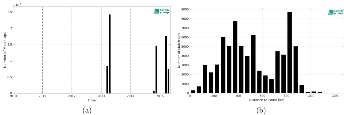
Figure 1: Number of match-ups between TSG (CSIC-UTM) and Aquarius SSS L4 OI v5 - Monthly (IPRC) SSS as a function of time (a) and as function of the distance to coast (b) over the South Atlantic Ocean Pi-MEP region and for the full satellite product period.
