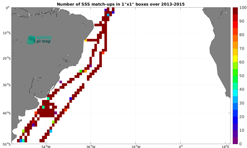
Figure 4: Number of SSS match-ups between TSG (CSIC-UTM) SSS and the Aquarius SSS L4 OI v5 - Monthly (IPRC) SSS product for the South Atlantic Ocean Pi-MEP region over 1^\circ \times 1^\circ boxes and for the full satellite product period.
