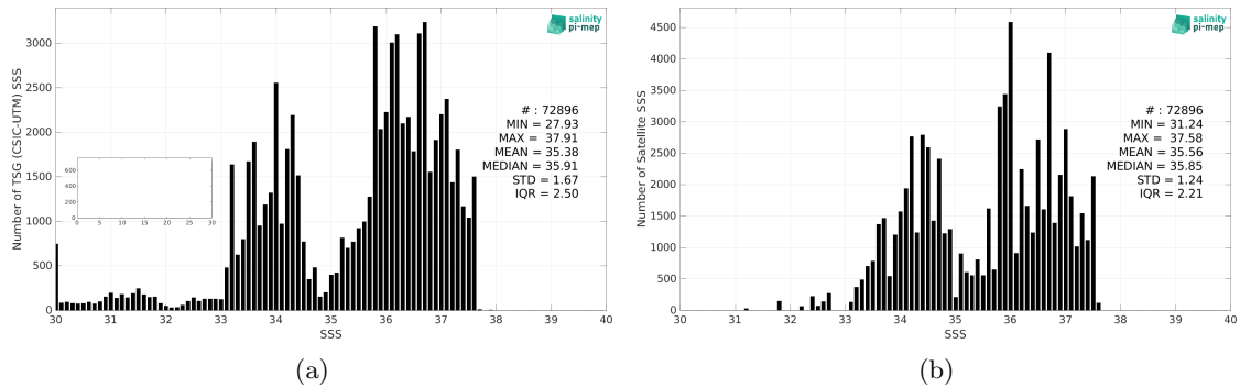
Figure 2: Histograms of SSS from TSG (CSIC-UTM) (a) and Aquarius SSS L4 OI v5 - Monthly (IPRC) (b) considering all match-up pairs per bins of 0.1 over the South Atlantic Ocean Pi-MEP region and for the full satellite product period.
