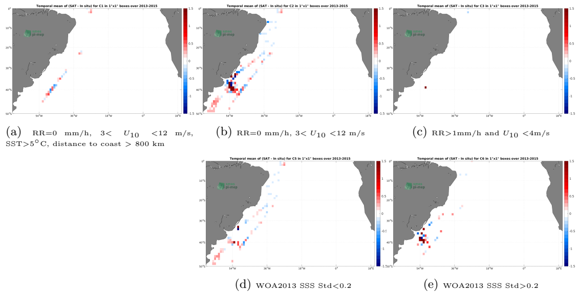
Figure 12: Temporal mean gridded over spatial boxes of size 1^\circ \times 1^\circ of \Delta SSS (Aquarius SSS L4 OI v5 - Monthly (IPRC) - TSG (CSIC-UTM)) for 5 different subdatasets corresponding to:RR=0 mm/h, 3 < U_{10} < 12 m/s, SST >5^\circ\text{C} , distance to coast > 800 km (a), RR=0 mm/h, 3 < U_{10} < 12 m/s (b), RR >1 mm/h and U_{10} < 4 m/s (c), WOA2013 SSS Std <0.2 (d), WOA2013 SSS Std >0.2 (e).
