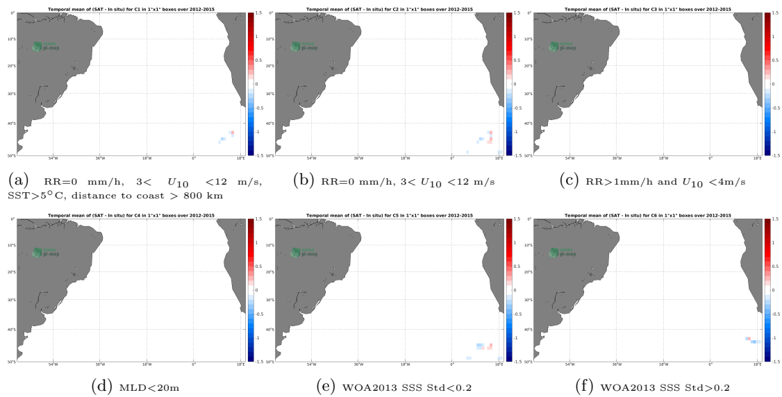
Figure 12: Temporal mean gridded over spatial boxes of size 1^{\circ}\times 1^{\circ} of \Delta\text{SSS} (Aquarius SSS L4 OI v5 - Monthly (IPRC) - Sea mammals) for 6 different subdatasets corresponding to: RR=0 mm/h, 3 < U_{10} < 12 m/s, SST > 5^{\circ}\text{C} , distance to coast > 800 km (a), RR=0 mm/h, 3 < U_{10} < 12 m/s (b), RR > 1\text{mm/h} and U_{10} < 4\text{m/s} (c), MLD < 20\text{m} (d), WOA2013 SSS Std < 0.2 (e), WOA2013 SSS Std > 0.2 (f).
