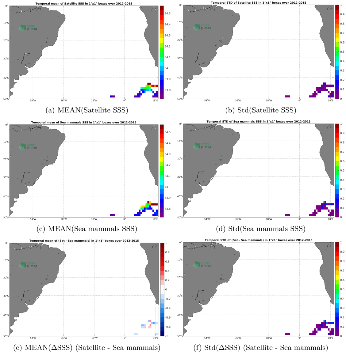
Figure 6: Temporal mean (left) and Std (right) of SSS from Aquarius SSS L4 OI v5 - Monthly (IPRC) (top), Sea mammals (middle), and of \Delta SSS (Satellite - Sea mammals). Only match-up pairs are used to generate these maps.
