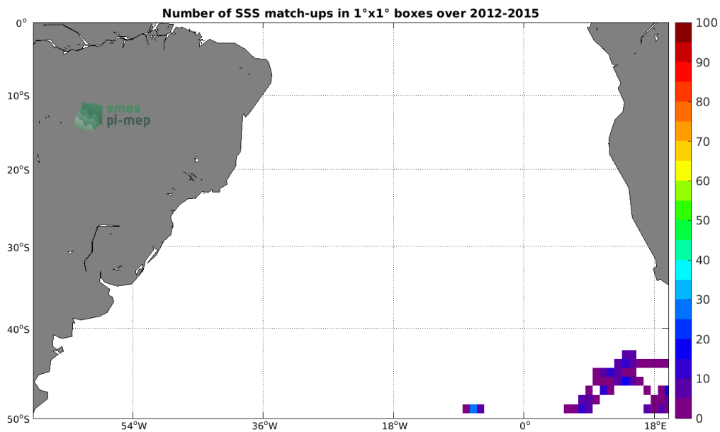
Figure 4: Number of SSS match-ups between Sea mammals SSS and the Aquarius SSS L4 OI v5 - Monthly (IPRC) SSS product for the South Atlantic Ocean Pi-MEP region over 1^\circ \times 1^\circ boxes and for the full satellite product period.
