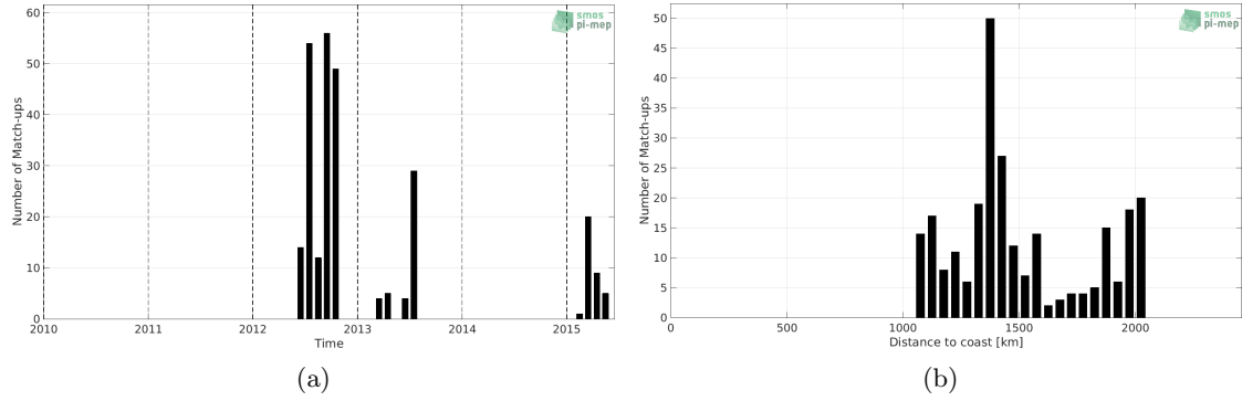
Figure 1: Number of match-ups between Sea mammals and Aquarius SSS L4 OI v5 - Monthly (IPRC) SSS as a function of time (a) and as function of the distance to coast (b) over the South Atlantic Ocean Pi-MEP region and for the full satellite product period.
