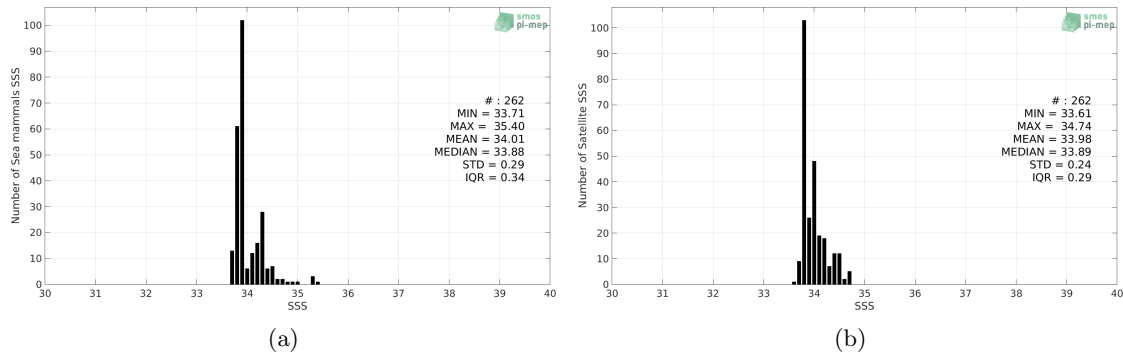
Figure 2: Histograms of SSS from Sea mammals (a) and Aquarius SSS L4 OI v5 - Monthly (IPRC) (b) considering all match-up pairs per bins of 0.1 over the South Atlantic Ocean Pi-MEP region and for the full satellite product period.
