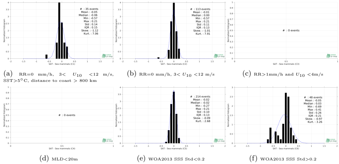
Figure 13: Normalized histogram of \Delta SSS (Aquarius-L4-IPRC-V5-MONTHLY - Sea mammals) for 6 different subdatasets corresponding to: RR=0 mm/h, 3 < U_{10} < 12 m/s, SST>5°C, distance to coast > 800 km (a), RR=0 mm/h, 3 < U_{10} < 12 m/s (b), RR>1mm/h and U_{10} < 4 m/s (c), MLD<20m (d), WOA2013 SSS Std<0.2 (e), WOA2013 SSS Std>0.2 (f).
