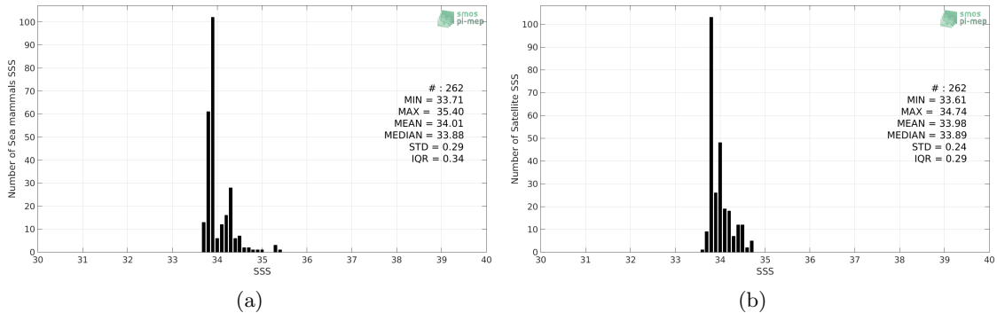
Figure 2: Histograms of SSS from Sea mammals (a) and Aquarius-L4-IPRC-V5-MONTHLY (b) considering all match-up pairs per bins of 0.1 over the South Atlantic Ocean Pi-MEP region and for the full satellite product period.
