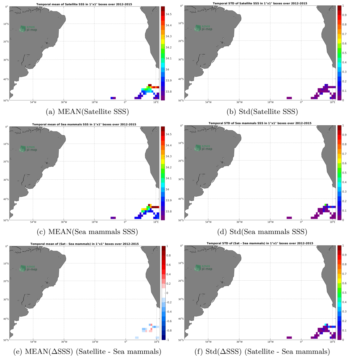
Figure 6: Temporal mean (left) and Std (right) of SSS from Aquarius-L4-IPRC-V5-MONTHLY (top), Sea mammals (middle), and of \Delta SSS (Satellite - Sea mammals). Only match-up pairs are used to generate these maps.
