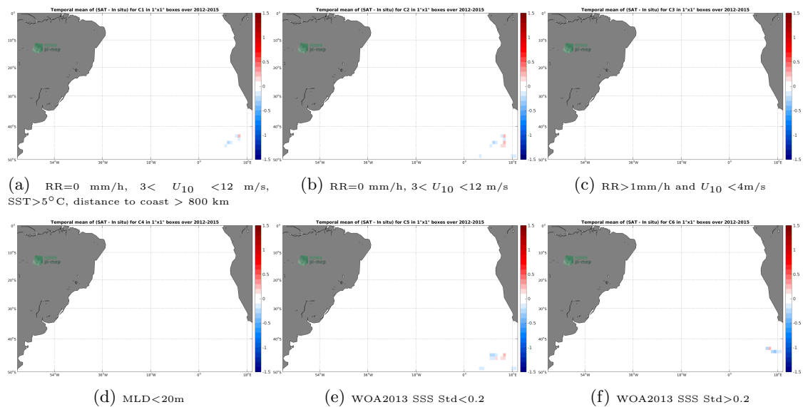
Figure 12: Temporal mean gridded over spatial boxes of size 1^{\circ}\times 1^{\circ} of \Delta\text{SSS} (Aquarius-L4-IPRC-V5-MONTHLY - Sea mammals) for 6 different subdatasets corresponding to:RR=0 mm/h, 3 < U_{10} < 12 m/s, SST >5^{\circ}\text{C} , distance to coast > 800 km (a), RR=0 mm/h, 3 < U_{10} < 12 m/s (b), RR >1 mm/h and U_{10} < 4 m/s (c),MLD <20 m (d),WOA2013 SSS Std <0.2 (e),WOA2013 SSS Std >0.2 (f).
