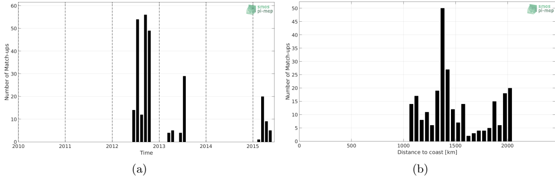
Figure 1: Number of match-ups between Sea mammals and Aquarius-L4-IPRC-V5-MONTHLY SSS as a function of time (a) and as function of the distance to coast (b) over the South Atlantic Ocean Pi-MEP region and for the full satellite product period.
