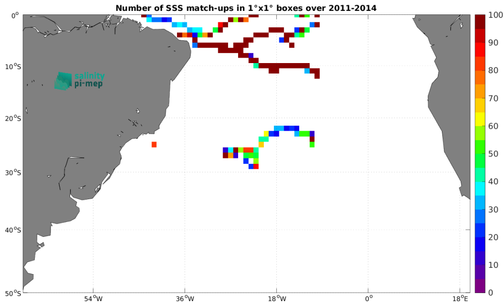
Figure 4: Number of SSS match-ups between Surface drifters SSS and the Aquarius SSS L4 OI v5 - Monthly (IPRC) SSS product for the South Atlantic Ocean Pi-MEP region over 1^\circ \times 1^\circ boxes and for the full satellite product period.
