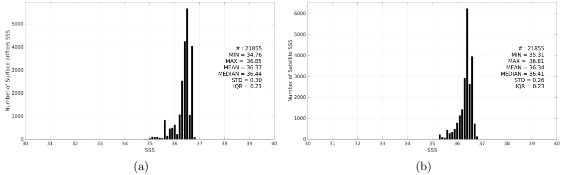
Figure 3: Histograms of SSS from Surface drifters (a) and Aquarius SSS L4 OI v5 - Monthly (IPRC) (b) considering all match-up pairs per bins of 0.1 over the South Atlantic Ocean Pi-MEP region and for the full satellite product period.
