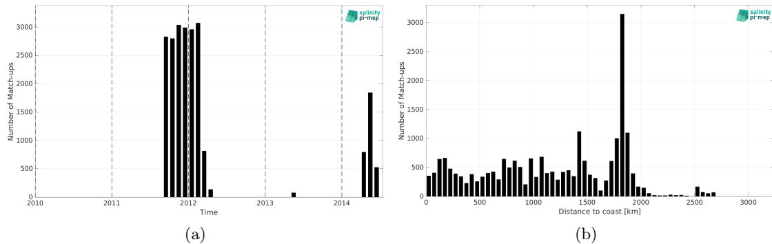
Figure 2: Number of match-ups between Surface drifters and Aquarius SSS L4 OI v5 - Monthly (IPRC) SSS as a function of time (a) and as function of the distance to coast (b) over the South Atlantic Ocean Pi-MEP region and for the full satellite product period.
