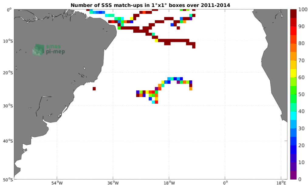
Figure 3: Number of SSS match-ups between Surface drifters SSS and the Aquarius SSS L4 OI v5 - Monthly (IPRC) SSS product for the South Atlantic Ocean Pi-MEP region over 1^\circ \times 1^\circ boxes and for the full satellite product period.
