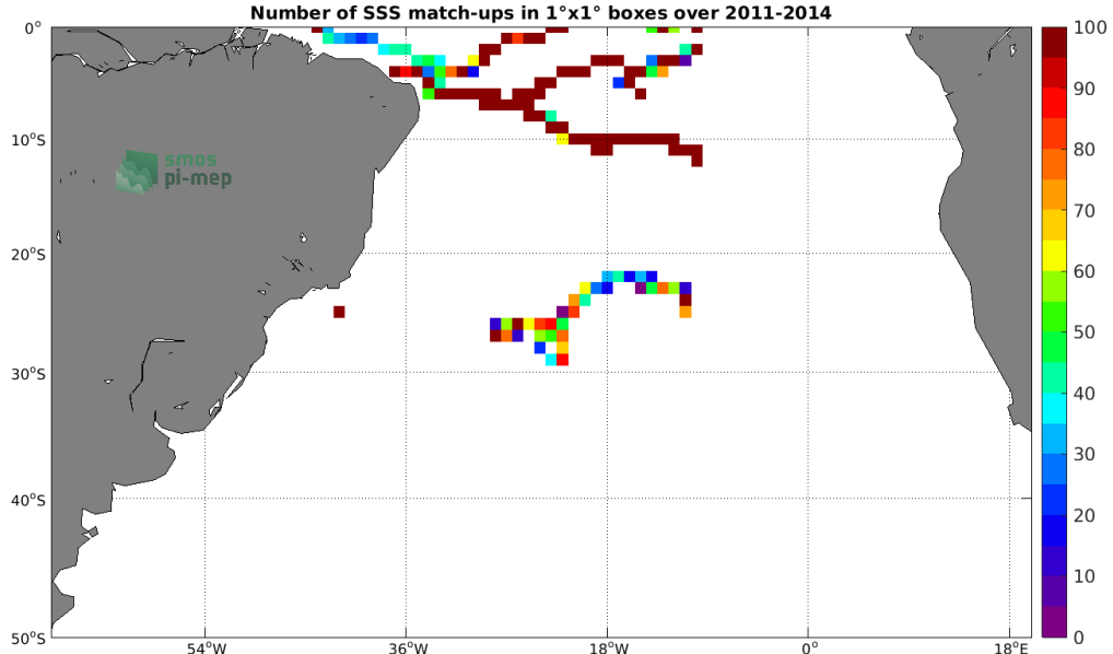
Figure 3: Number of SSS match-ups between Surface drifters SSS and the Aquarius SSS L4 OI v5 - Monthly (IPRC) SSS product for the South Atlantic Ocean Pi-MEP region over 1^\circ \times 1^\circ boxes and for the full satellite product period.
