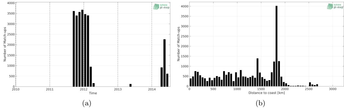
Figure 1: Number of match-ups between Surface drifters and Aquarius SSS L4 OI v5 - Monthly (IPRC) SSS as a function of time (a) and as function of the distance to coast (b) over the South Atlantic Ocean Pi-MEP region and for the full satellite product period.
