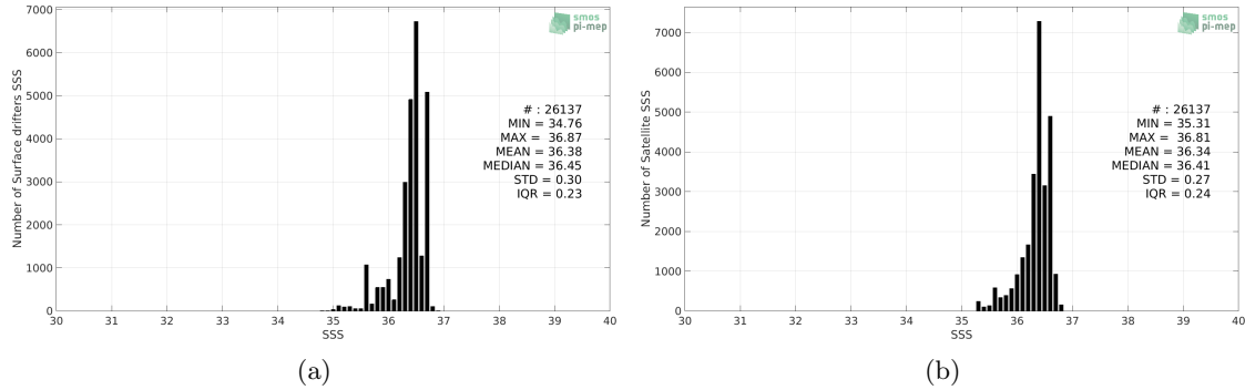
Figure 2: Histograms of SSS from Surface drifters (a) and Aquarius SSS L4 OI v5 - Monthly (IPRC) (b) considering all match-up pairs per bins of 0.1 over the South Atlantic Ocean Pi-MEP region and for the full satellite product period.
