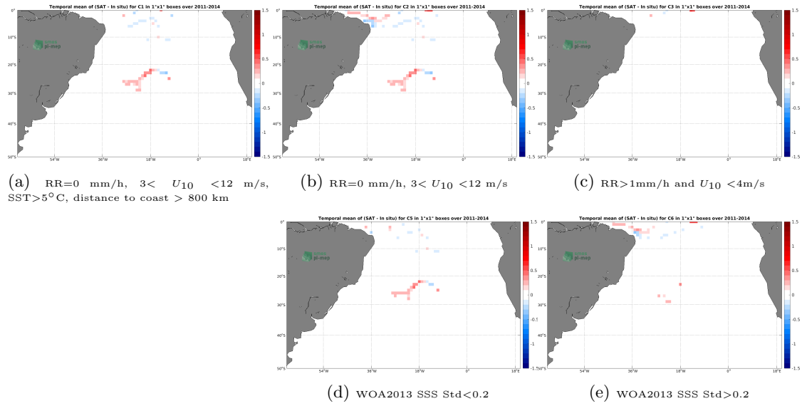
Figure 11: Temporal mean gridded over spatial boxes of size 1^\circ \times 1^\circ of \Delta SSS (Aquarius SSS L4 OI v5 - Monthly (IPRC) - Surface drifters) for 5 different subdatasets corresponding to: RR=0 mm/h, 3 < U_{10} < 12 m/s, SST > 5^\circ C , distance to coast > 800 km (a), RR=0 mm/h, 3 < U_{10} < 12 m/s (b), RR > 1 mm/h and U_{10} < 4 m/s (c), WOA2013 SSS Std < 0.2 (d), WOA2013 SSS Std > 0.2 (e).
