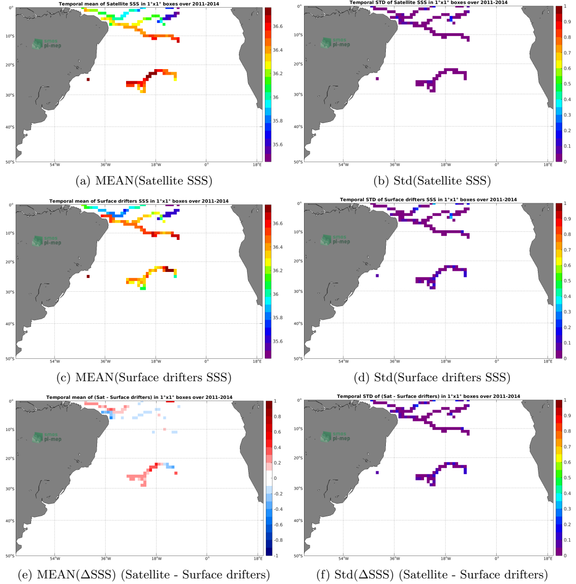
Figure 5: Temporal mean (left) and Std (right) of SSS from Aquarius SSS L4 OI v5 - Monthly (IPRC) (top), Surface drifters (middle), and of \Delta SSS (Satellite - Surface drifters). Only match-up pairs are used to generate these maps.
